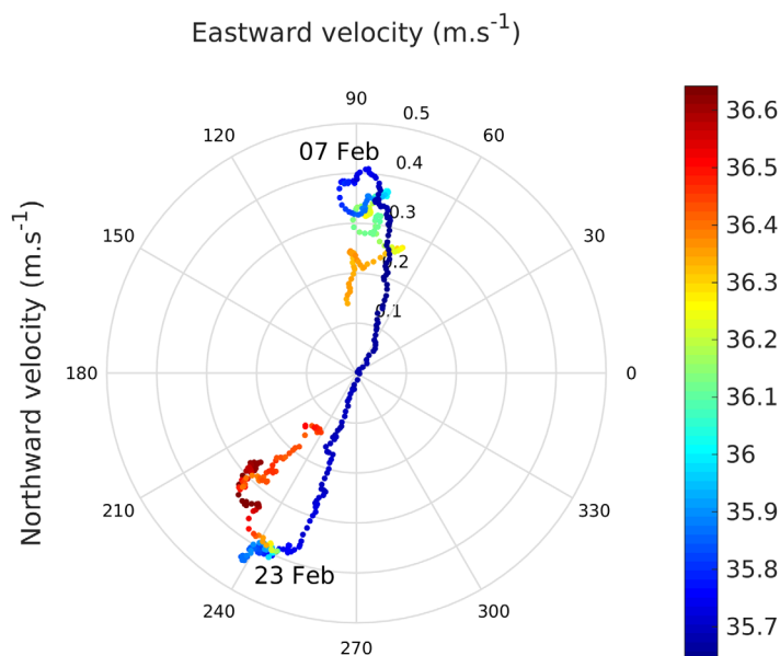
Figure 3. Hodograph of the observed currents averaged between 40 and 100 m depth for the period 26 January to 6 March 2010. The color corresponds to the salinity averaged between 40 and 100 m depth. The two dates correspond to the occurrence of the strongest northward and southward velocities.
