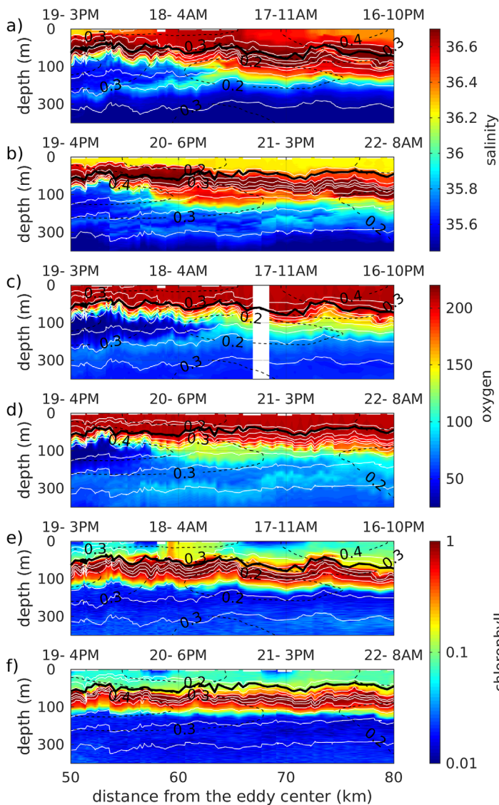
Figure 6. (a and b) Glider salinity, (c and d) oxygen ( \mu\text{mol L}^{-1} ), and (e and f) fluorescence ( \text{mg m}^{-3} ) data for the two crossing of the eddy rim from 16 to 22 March (the day of March and the time are indicated on top of the sections). Note that the fluorescence is plotted on a log scale. White lines represent isopycnals, black dashed lines the velocity contours and the thick black line the depth of the mixed layer. Note that the vertical scale is not linear and highlights the 0–100 m part.
