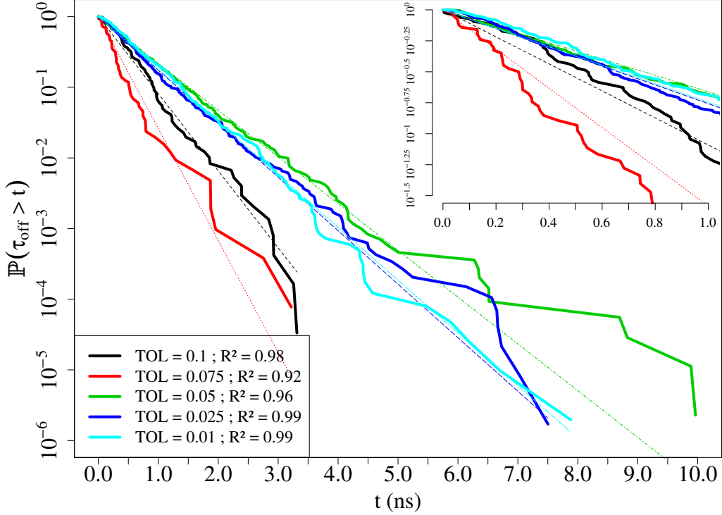
Figure 11: Distribution of the dissociation time \tau_{\text{off}} for the complex FKBP–DMSO, estimated using the Gen. ParRep method, at different levels of tolerance \text{TOL} = \{0.1, 0.075, 0.05, 0.025, 0.01\} . The top-right inset is a zoom for t < 1.0 ns, and dashed straight lines (for which the R^2 coefficient of determination is given) denote the expected quasi-exponential distribution for large t : \ln \mathbb{P}(\tau_{\text{off}} > t) = -t/\mathbb{E}(\tau_{\text{off}}) . See Table 3 for quantitative values of: \mathbb{E}(\tau_{\text{off}}) , N , n and the 95% confidence interval.
