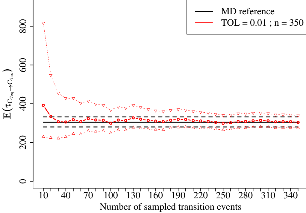
Figure 6: Convergence of \mathbb{E}(\tau_{C_{7eq} \rightarrow C_{7ax}}) (solid lines) for Gen. ParRep sampled values from Figure 5, when considering only the first m sampled values among n = 350 (abscissa). Dashed lines correspond to the 95% confidence interval.
