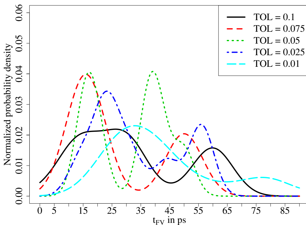
Figure 13: Kernel Density Estimation of the distribution of t_{F-V} , obtained for tolerance levels of TOL = \{0.1, 0.075, 0.05, 0.025, 0.01\} (datasets from Figure 11 and Table 3).
