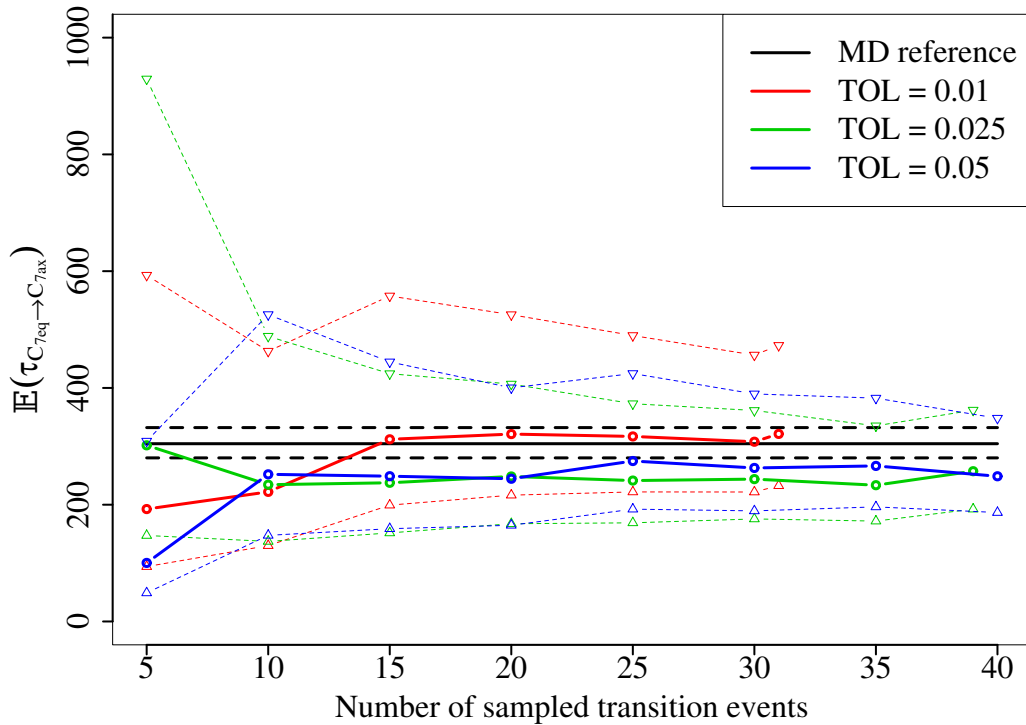
Figure 4: Convergence of \mathbb{E}(\tau_{C_{7\text{eq}} \rightarrow C_{7\text{ax}}}) (plain lines) to the MD reference (black lines), for Gen. ParRep sampled values (red, green and blue lines), when considering only the first m of the n = \{31, 39, 40\} samples (abscissa), for \text{TOL} levels of respectively \{0.01, 0.025, 0.05\} . Dashed lines correspond to the 95% confidence interval; The number of Gen. ParRep replicas was fixed at N = 224 .
