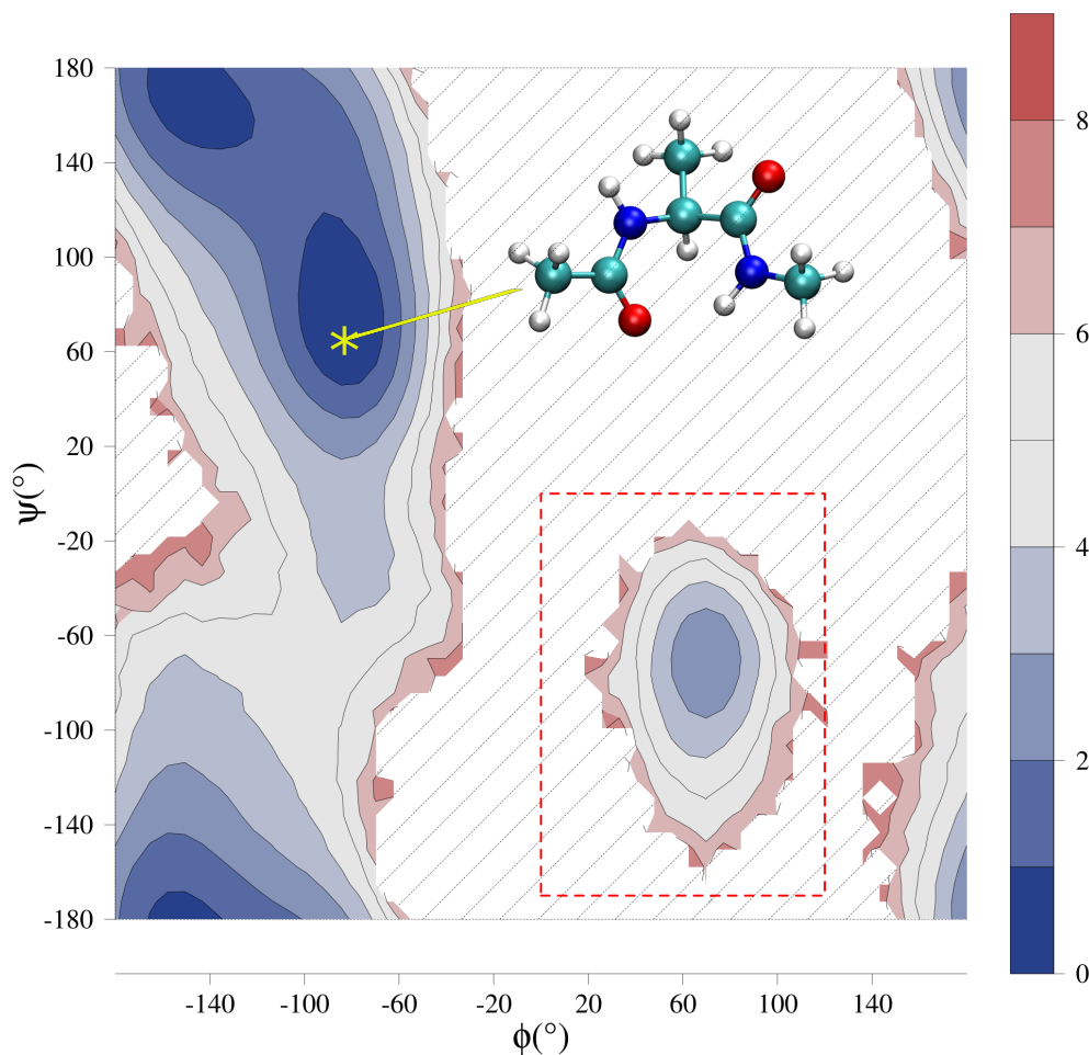
Figure 3: Alanine dipeptide : definition of ParRep domains based on a free energy surface (color coded, in kcal/mol, dashed oblique lines correspond to unsampled areas), constructed from the long MD reference simulation. The red rectangle corresponding to \phi \in [0; 120] and \psi \in [-170; 0] is used as a threshold defining the C_{7_{\text{ax}}} state (see subsection 4.1 for details). The yellow cross corresponds to the starting configuration for either Gen. ParRep or serial MD simulations.
