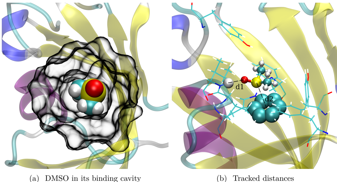
Figure 9: On the left a closer view of the DMSO ligand in its binding cavity: favorable interactions between the O or S atoms and surface residues, together with the little available space around the ligand, are responsible for metastability. On the right, surrounding residues within the cavity are represented: in order to detect the dissociation event two distances are tracked for defining the bound state (see the Gen. ParRep setup paragraph for details).
