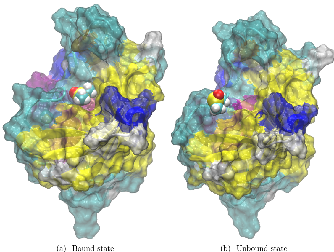
Figure 8: Illustration of the FKBP–DMSO complex, corresponding to the RCSB-PDB entry “1D7H” : on the left the undissociated (“bound”) state used as starting configuration for all the simulations; on the right the target dissociated (“unbound”) state characterized by a \tau_{\text{off}} dissociation time.
