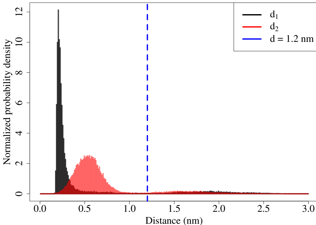
Figure 10: Histogram distribution of the two d_1 and d_2 distances as defined in Figure 9 (b), for 30 ns of plain Langevin dynamics.
