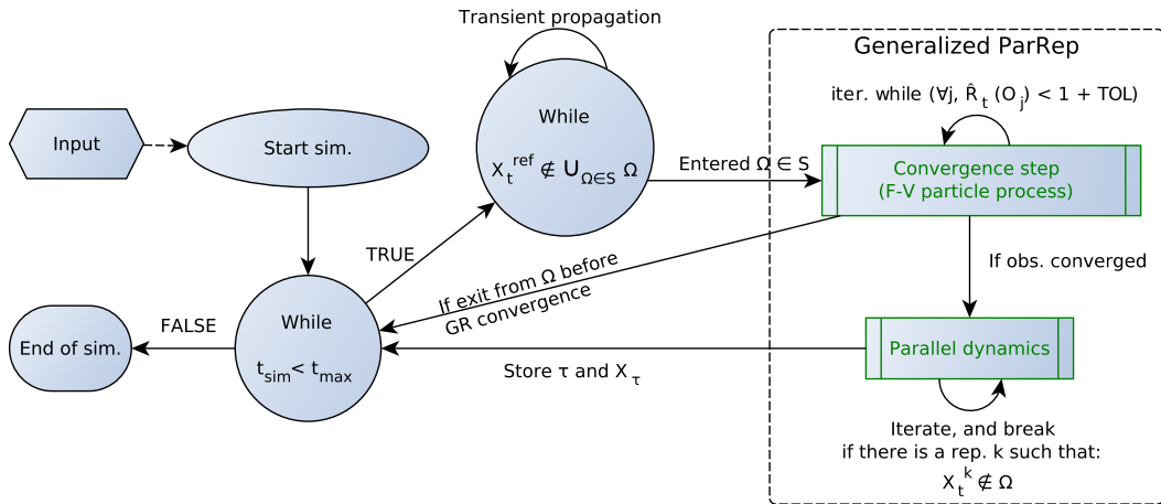
Figure 1: Diagram view of the generalized ParRep [43] algorithm. After setup, the first step (Transient propagation) is to iterate the reference walker until X_t enters a defined state \Omega (if the states define a partition of the configuration space, this first part of the algorithm is not required); then the Gen. ParRep procedure (right frame) is executed, starting with the Convergence step, until either: (i) the reference walker exits before convergence of the G-R statistics is observed, or (ii) convergence of the G-R observables is obtained before the reference walker exits. In the later case simulation proceeds to the Parallel dynamics step, until an exit event from \Omega is observed, generating a sample of (\tau, X_\tau) . After the parallel phase (or if X_t exited \Omega before convergence), the reference walker performs once again the Transient propagation procedure, until entering a valid state \Omega , and the Gen. ParRep procedure is iterated once again. This is repeated until the total simulation time t_{\text{sim}} reaches a user defined value t_{\text{max}} , where the program stops. The two frames colored in green are parts of the algorithm fully exploiting the N available CPU cores.
