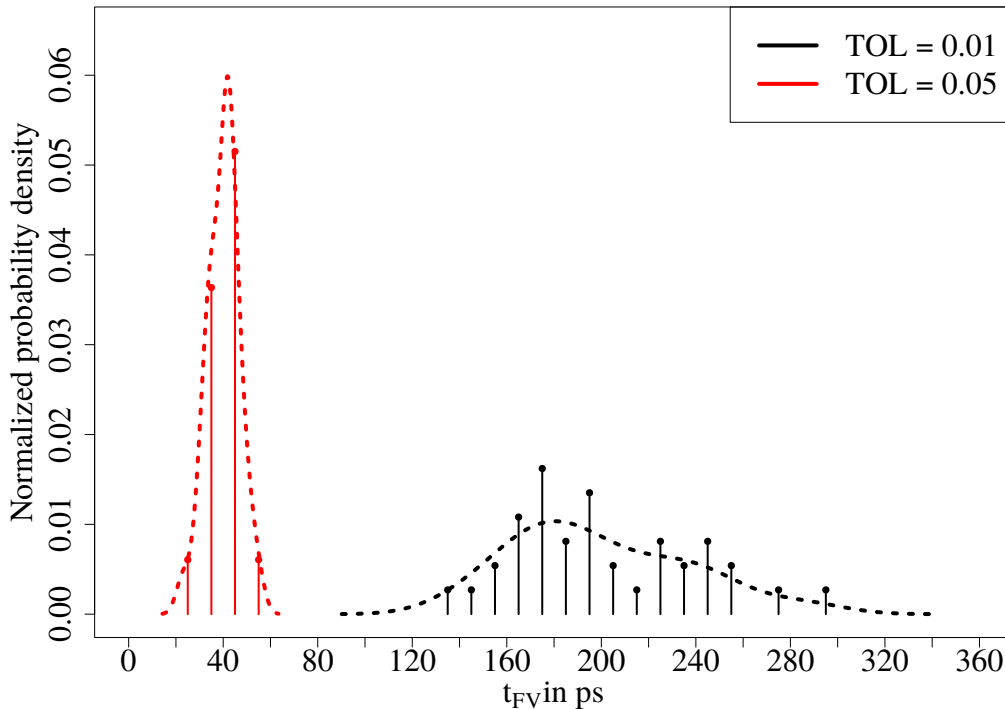
Figure 7: Histogram distribution (vertical lines) of t_{F-V} , obtained for two different tolerance levels of \text{TOL} = \{0.01, 0.05\} (two datasets from Figure 4): t_{F-V} corresponds to the simulation time before one assumes that the samples are distributed according to the QSD (see subsection 2.4). The dashed lines correspond to a Kernel Density Estimation [80, 81] smoothing.
