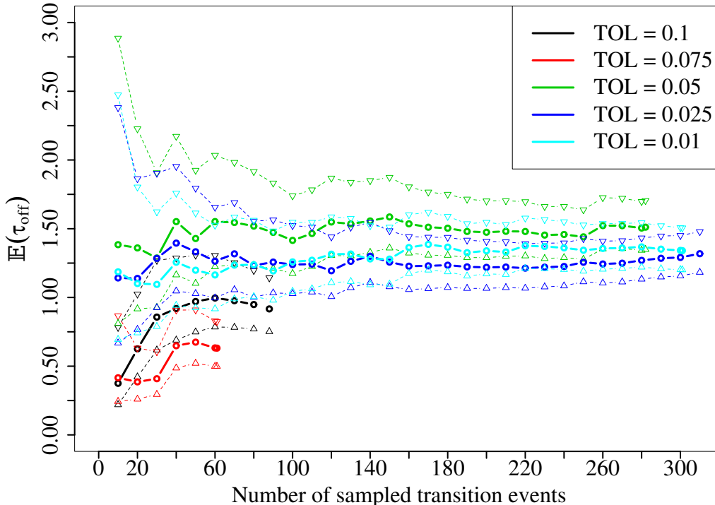
Figure 12: Convergence of \mathbb{E}(\tau_{\text{off}}) for the datasets from Figure 11 and Table 3. Dashed lines correspond to the 95% confidence interval.
