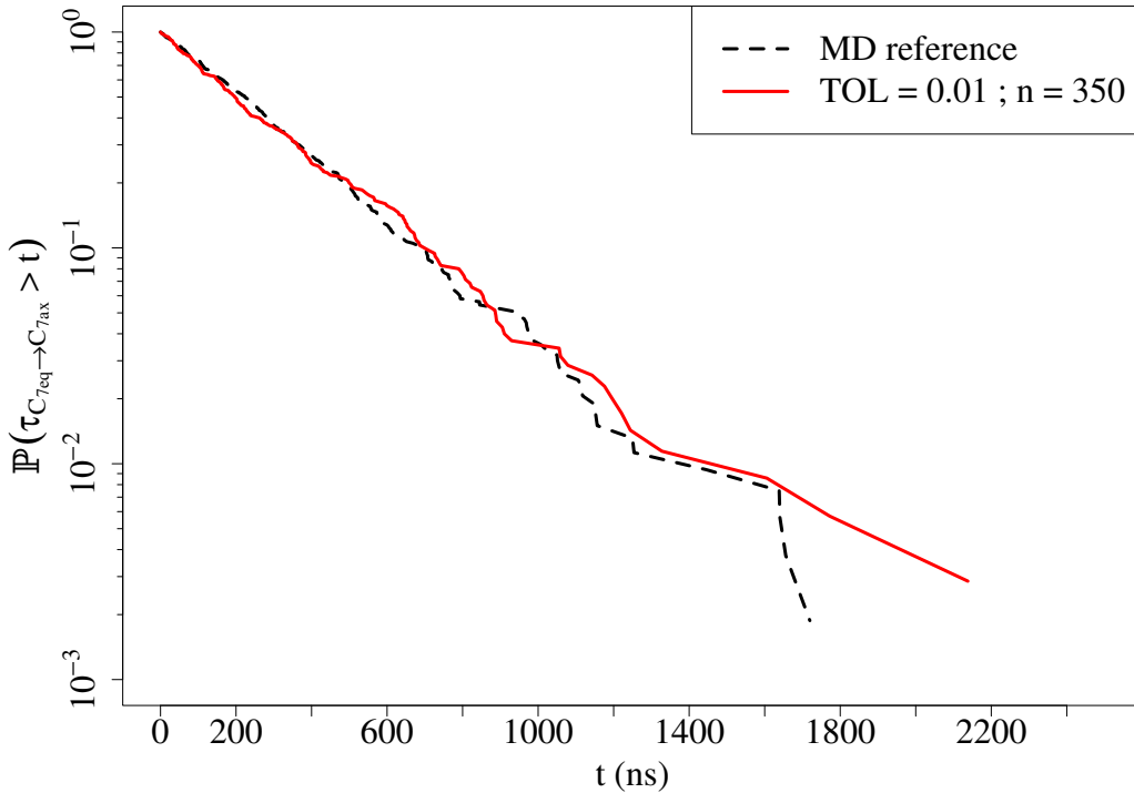
Figure 5: Distribution of Gen. ParRep sampled values of \tau_{C_{7\text{eq}} \rightarrow C_{7\text{ax}}} for \text{TOL} = 0.01 , for N = 224 , and a number of \tau values generated n = 350 .
