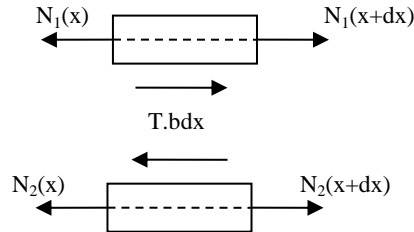
Figure 3. Free body diagram of infinitesimal pieces included between x and x+dx of both adherends in the overlap region. Subscript 1 (2) refers to the upper (lower) adherend.
