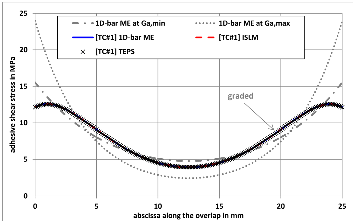
Figure 12. Adhesive shear stress distribution along the overlap associated with TC#1 for the 1D-bar analyses.
