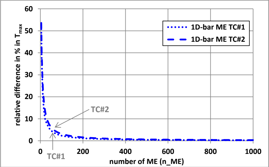
Figure 10. Relative difference in % in the maximal adhesive provided the 1D-bar ME analysis from the one by 1D-bar TEPS analysis as function of the number of MEs for both TC#1 and TC#2.
