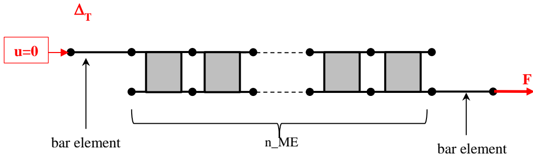
Figure 5. ME model of the FGA single lap joint.
