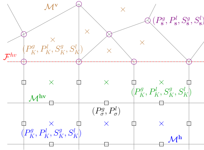
Figure 10: 2D mesh with examples of discrete unknowns in the set U_{\mathcal{D}} for the two-phase flow model.
