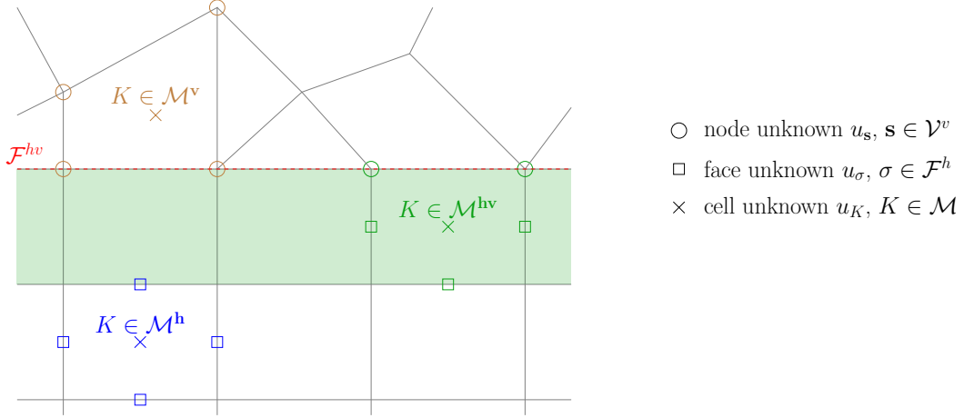
Figure 1: Example of a 2D mesh with the partition of the cells between the VAG cells K \in \mathcal{M}^v , the HFV cells K \in \mathcal{M}^h and the interface cells K \in \mathcal{M}^{hv} . Examples of cell (crosses), node (circles) and face (squares) degrees of freedom of \text{dof}_{\mathcal{D}} in the VAG, HFV and interface regions.
