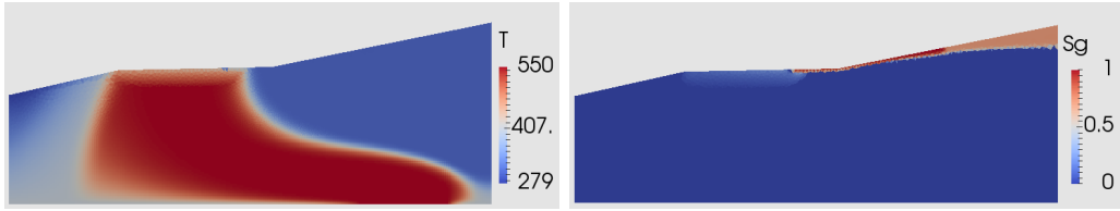
Figure 20: Temperature (in K) and gas saturation at final time (650 years) obtained with the VAG-TPFA scheme on the Cartesian-triangular mesh.
