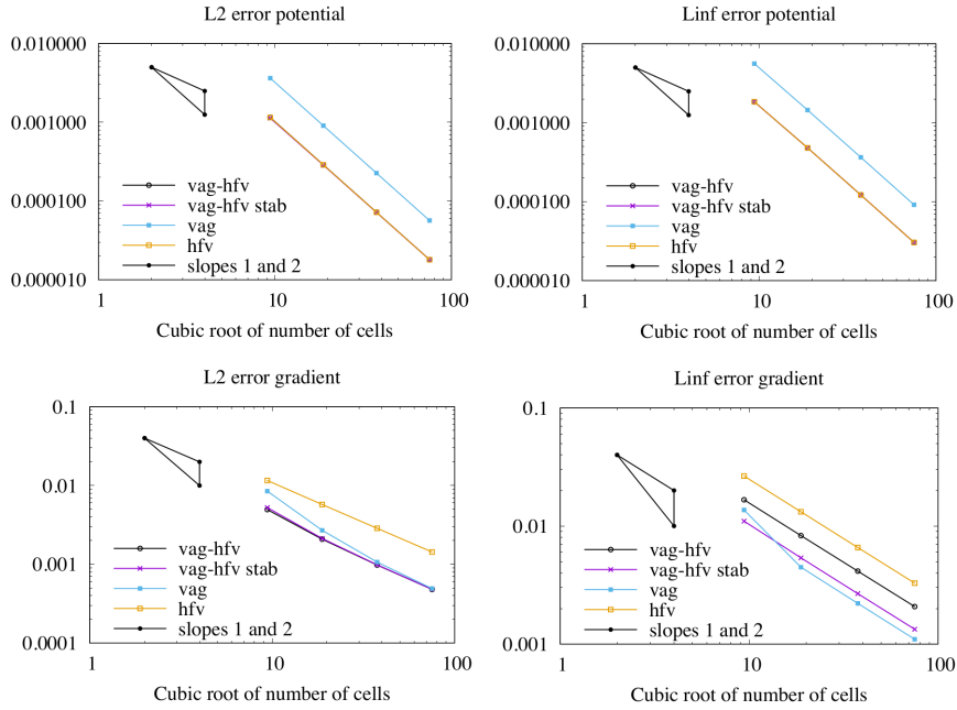
Figure 5: Convergence in L^2 norm (left) and in L^\infty norm (right) of the potential (above) and of the gradient (below) on the family of hybrid meshes and for the VAG, HFV, VAG-HFV and the stabilised VAG-HFV schemes.
