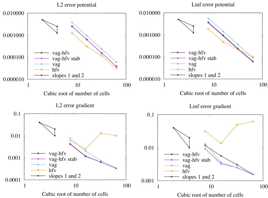
Figure 3: Convergence in L^2 norm (left) and in L^\infty norm (right) of the potential (above) and of the gradient (below) on the family of hexahedral meshes and for the VAG, HFV, VAG-HFV and the stabilised VAG-HFV schemes.
