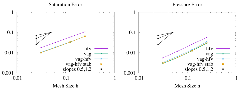
Figure 14: Convergence in space time discrete L^1 norm of the saturation and the non-wetting pressure on the family of Cartesian meshes with red black coloring and for the VAG, HFV, VAG-HFV and the stabilised VAG-HFV schemes.
