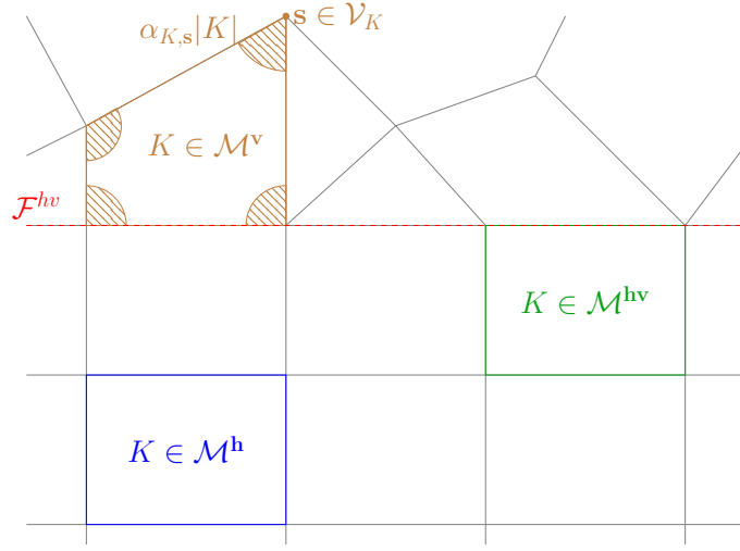
Figure 9: Example of a 2D mesh with the distribution of the volumes \alpha_{K,s}|K| at each node s \in \mathcal{V}_K of the cell K \in \mathcal{M}^v in the case of a single rock type.
