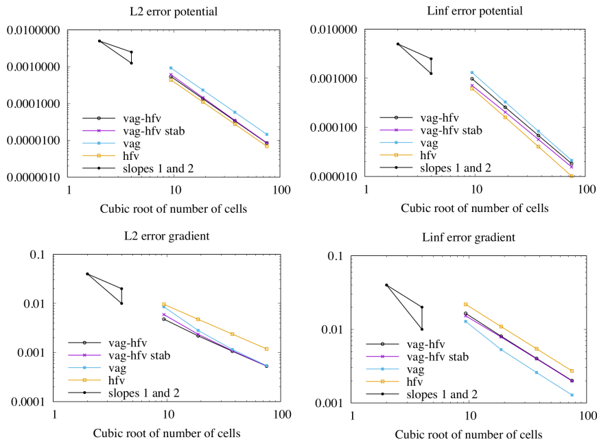
Figure 6: Convergence in L^2 norm (left) and in L^\infty norm (right) of the potential (above) and of the gradient (below) on the family of hybrid meshes (hexahedral and pyramidal cells) with anisotropic permeability and for the VAG, HFV, VAG-HFV and the stabilised VAG-HFV schemes.
