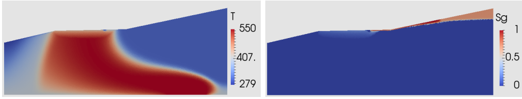
Figure 19: Temperature (in K) and gas saturation at final time (650 years) obtained with the TPFA scheme on the Voronoi mesh.
