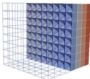
Figure 12: Hybrid mesh obtained for N = 8 and composed of cubes in the HFV subdomain \Omega \setminus \overline{\Omega^v} and of pyramids in the VAG subdomain \Omega^v = (0.5, 1) \times (0, 1)^2 .
