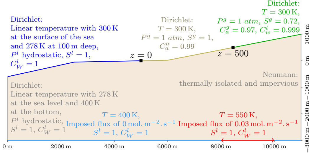
Figure 15: Illustration of the two dimensional geothermal reservoir and of the various conditions applied at its boundary.
