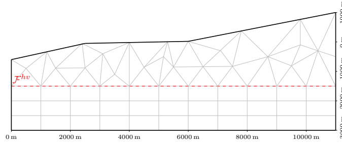
Figure 16: Coarse hybrid Cartesian-triangular mesh.
