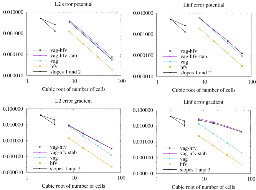
Figure 8: Convergence in L^2 norm (left) and in L^\infty norm (right) of the potential (above) and of the gradient (below) on the family of Cartesian meshes and for the VAG, HFV, VAG-HFV and the stabilised VAG-HFV schemes.
