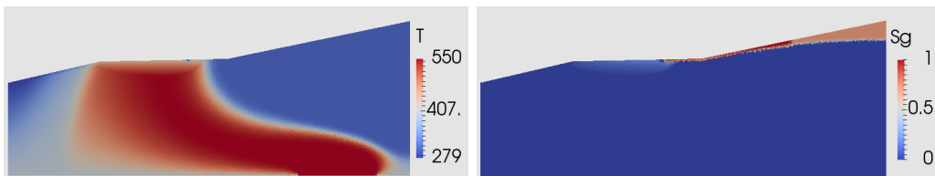
Figure 18: Temperature (in K) and gas saturation at final time (650 years) obtained with the VAG scheme on the triangular mesh.
