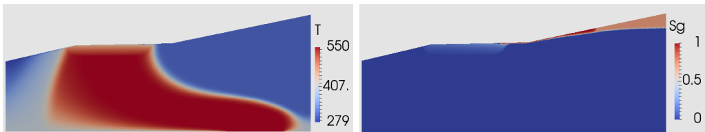
Figure 17: Reference temperature (in K) and gas saturation at final time (650 years) obtained with the refined Cartesian-Voronoi mesh combined with the VAG-TPFA scheme.
