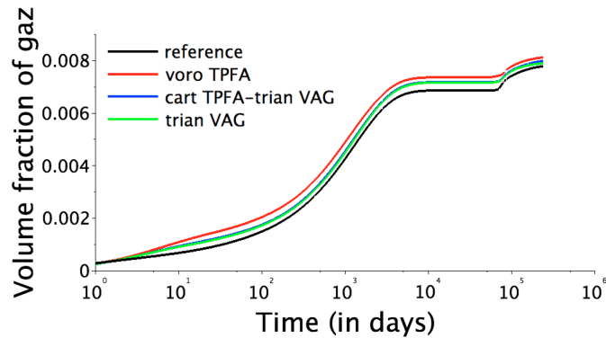
Figure 21: Ratio between the gas volume and the total pore volume as a function of time with log time scale for the various discretizations.
