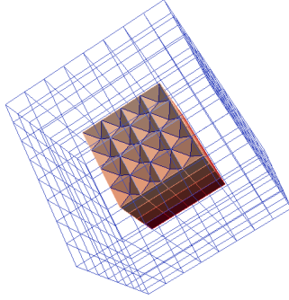
Figure 4: Hybrid mesh obtained for N = 8 and composed of cubes in the HFV subdomain \Omega \setminus \bar{\Omega}^v and of pyramids in the VAG subdomain \Omega^v = (0.25, 0.75)^3 .
