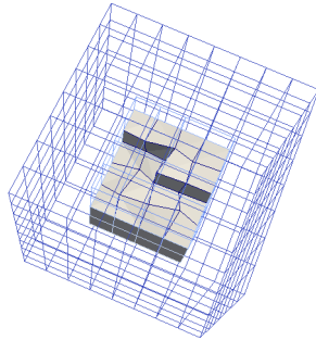
Figure 2: Hexahedral mesh obtained for N = 8 and composed of cubic cells in the HFV subdomain \Omega \setminus \overline{\Omega}^v and of randomly perturbed cubic cells in the VAG subdomain \Omega^v = (0.25, 0.75)^3 .
