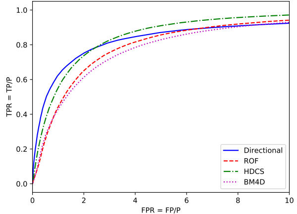
Fig. 4. Mean ROC curves over the 10 VascuSynth images with with a Poisson noise of gain g = 15 , for FPR values between 0 and 10. (Note that due to the sparsity of the images, the maximum TPR is reached for all methods only for a FPR around 100.)
