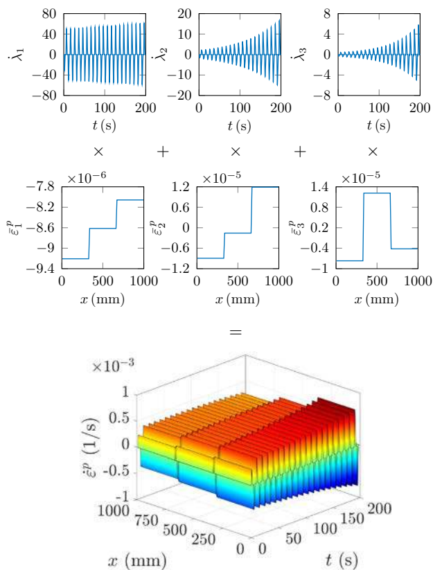
Fig. 5 Space-time modes needed to approximate \dot{\varepsilon}^P(x, t) in the bar under cyclic loading at convergence
