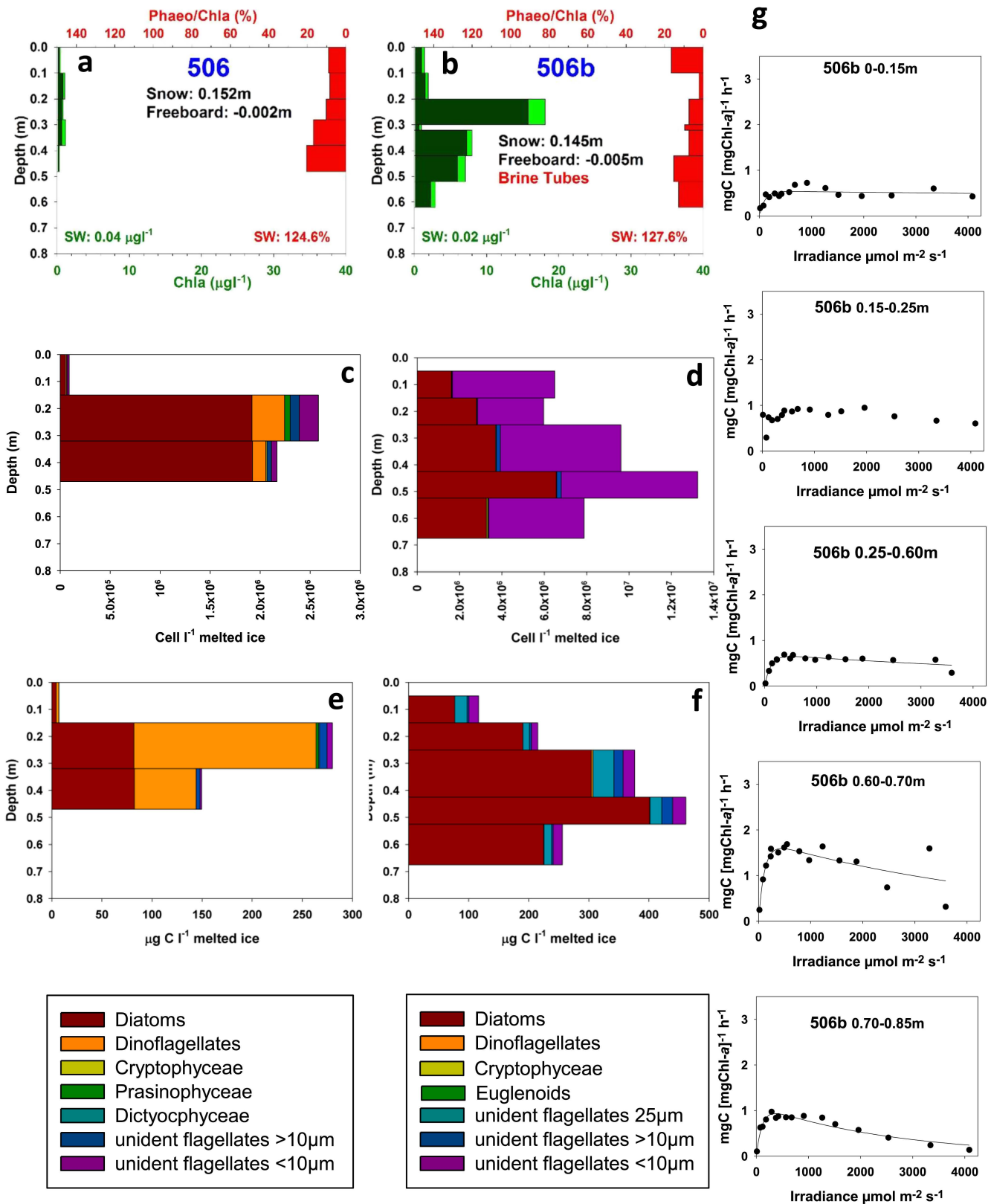
Figure 8. Biological characteristics at Station 506 (a and b are 4 days and 20 m apart)—(a and b) Chl-a (dark green = >10 \mu\text{m} ; light green = 0.8–10 \mu\text{m} ) and Phaeo-pigments to Chl-a ratio (%; red); (c and d) number of cells per liter of melted ice; (e and f) biomass in micrograms Carbon per liter of melted ice; (g) PI curves for five successive and continuous layers of station 506b. Note the difference in scales between 8c–8d and 8e–8f. See text for details.
