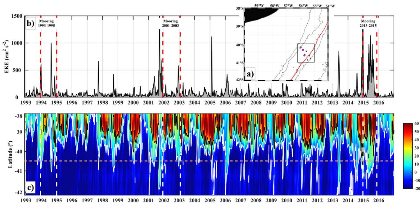
Figure 4. (a) Bottom topography and mooring locations. The 6,000, 5,000, 3,000, 1,000, and 300 m isobaths are represented with solid light grey contours, the 2,000 m contour is highlighted in red. (b) Surface Eddy Kinetic Energy estimated from MGP around mooring locations (black square in Figure 4a) over the period 1993–2016. (c) Absolute Dynamic Topography (ADT) along isobath 2000 m. The -5 and +30 cm ADT values corresponding to the SAF and BCF are marked with white and black lines, respectively. Mooring periods are indicated with vertical dashed lines. The dashed line at 40.5^{\circ} S corresponds to the intersection of Jason track #26 and the 2,000 m isobath.
