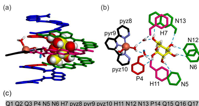
Fig. 4 (a) Side view of the solid-state structure of the complex formed between capsule M-2-Cu 2+ and β- D -mannopyranose 5 ; (b) top view showing the heterocycles that interact with the guest. Dashed blue lines indicate hydrogen bonds. Hydrogen bonding distances and angles can be found in the Supplementary Table S9. (c) Numbering of the monomers of sequence 2 used in this figure. Isobutoxy side chains and cavity-excluded solvent molecules and counterions are omitted for clarity. The capsule backbone is represented in sticks. Copper atoms are represented bronze scaled balls.
