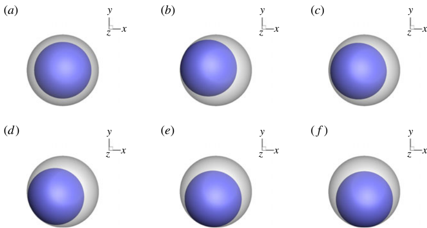
FIGURE 8. (Colour online) Trajectory of the centre of mass of the tank in the xy -plane and bubble positions at 6 different times with Bo_i = 1.16 , Bo_c = 0.116 and \tau_{fill} = 50\% .
