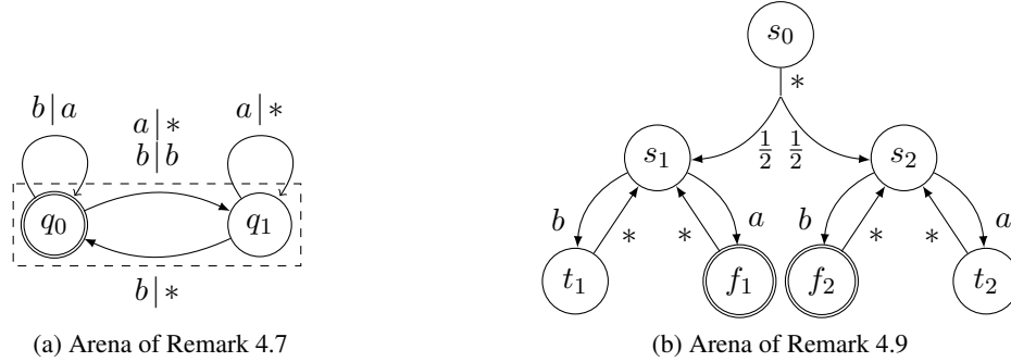
Figure 4: Arenas and beliefs
