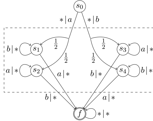
Figure 1: A concurrent arena where Adam is perfectly informed while Eve cannot distinguish states s_1, s_2, s_3 and s_4 .
