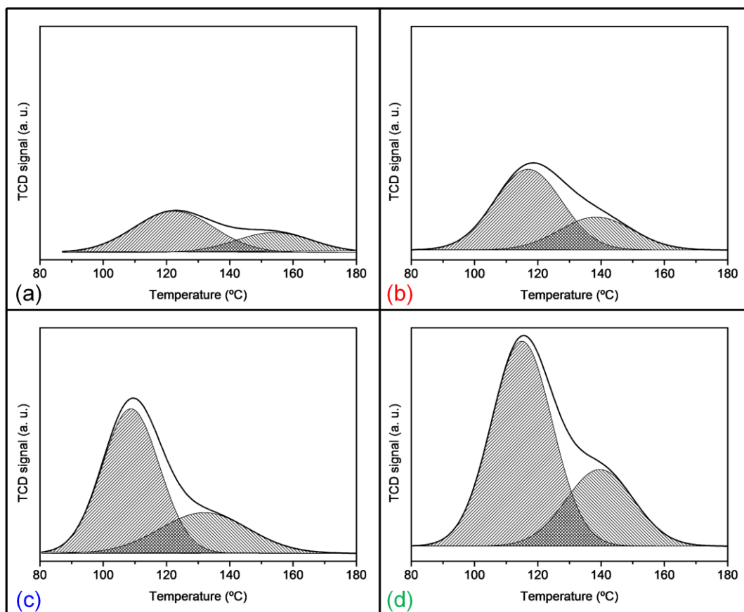
Figure 2 – Gaussian peak fitting to H_2 -TPR profiles of Pd(0.15)-HMOR (a), Pd(0.3)-HMOR (b), Pd(0.5)-HMOR (c) and Pd(0.7)-HMOR (d).
