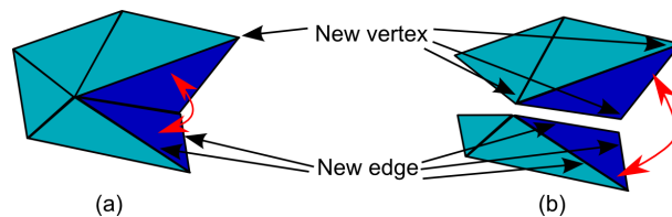
Figure 3: Oracle to detect if one new connected component appears after a face split. In (a), only one vertex and two edges split, so there is no new connected component. In (b), three vertices and three edges split, so one new connected component may appear.
