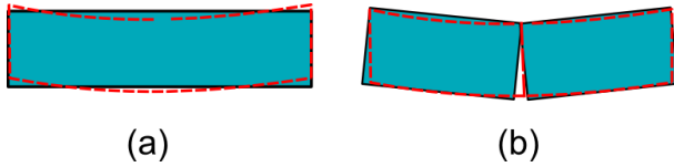
Figure 2: Discontinuity issue with Shape Matching. (a) A red block is deformed (red dotted line) and Shape Matching provides a position of the rigid reference (solid line). (b) A fracture occurs and the object is split. Shape Matching is separately applied on both connected components and results in a discontinuous state with respect to their positions in (a).
