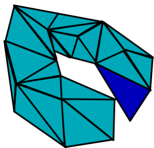
Figure 4: False positive of any local oracle. A local separation has occurred, so any local oracle predicts a new connected component, but the separated faces still belong to the same connected component (initially topologically-equivalent to a torus).
