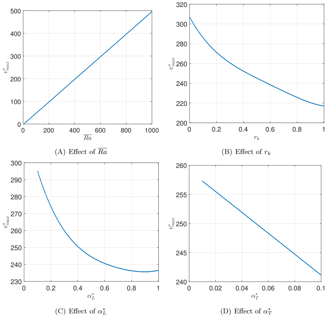
Fig. 10: Homogeneous case - Univariate effects of the input parameters on v_{max}^*
