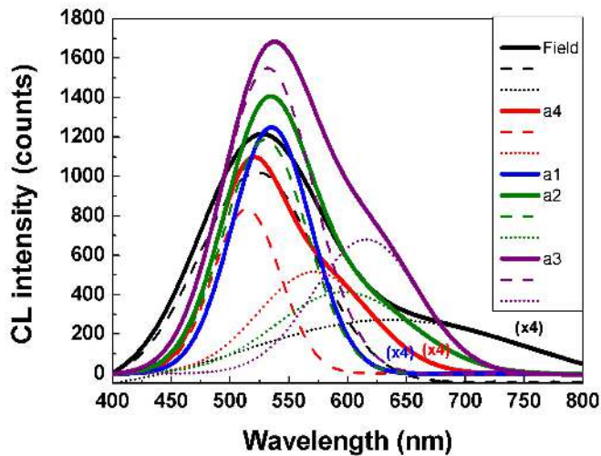
FIG. 6. Cathodoluminescence (CL) measurements at 77K on nanopylramids in patterns (a1) to (a4) and the field. All measurements come from one sample, meaning that all the patterned areas and the field experienced the same growth conditions.
