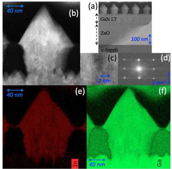
FIG. 5. STEM images of InGaN nanopillars. (a) HAADF image of 5 consecutive defect-free monocrystalline InGaN nanopillars grown by NSAG on top of 100 nm of low-temperature GaN, which was grown on 200nm-thick ZnO on c-sapphire. The FIB cut was realized along the [1\bar{1}00] direction. (b) HAADF zoom on one InGaN nanopillar, illustrating the single-crystal structure and absence of V-pits or threading dislocations which are common to all nanopillars. (c) A further HAADF zoom of the center of the InGaN nanopillar in Fig.5(b), revealing wurtzite structure. (d) FFT of Fig.5(c), confirming a hexagonal atomic arrangement in the InGaN. (e) EDX spectral map for the indium emission peak. (f) EDX image for the gallium emission peak.
