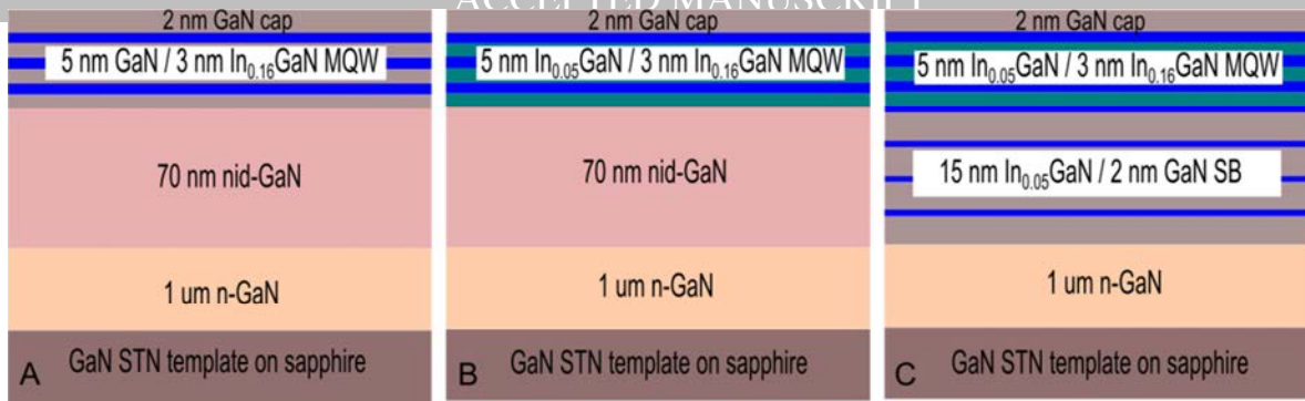
Fig. 1. Structure of the three samples under this study: reference sample A with GaN buffer and GaN barrier, reference sample B with GaN buffer and \text{In}_{0.05}\text{Ga}_{0.95}\text{N} barrier and final structure of sample C with semi-bulk \text{In}_{0.05}\text{Ga}_{0.95}\text{N} buffer and \text{In}_{0.05}\text{Ga}_{0.95}\text{N} barrier.
