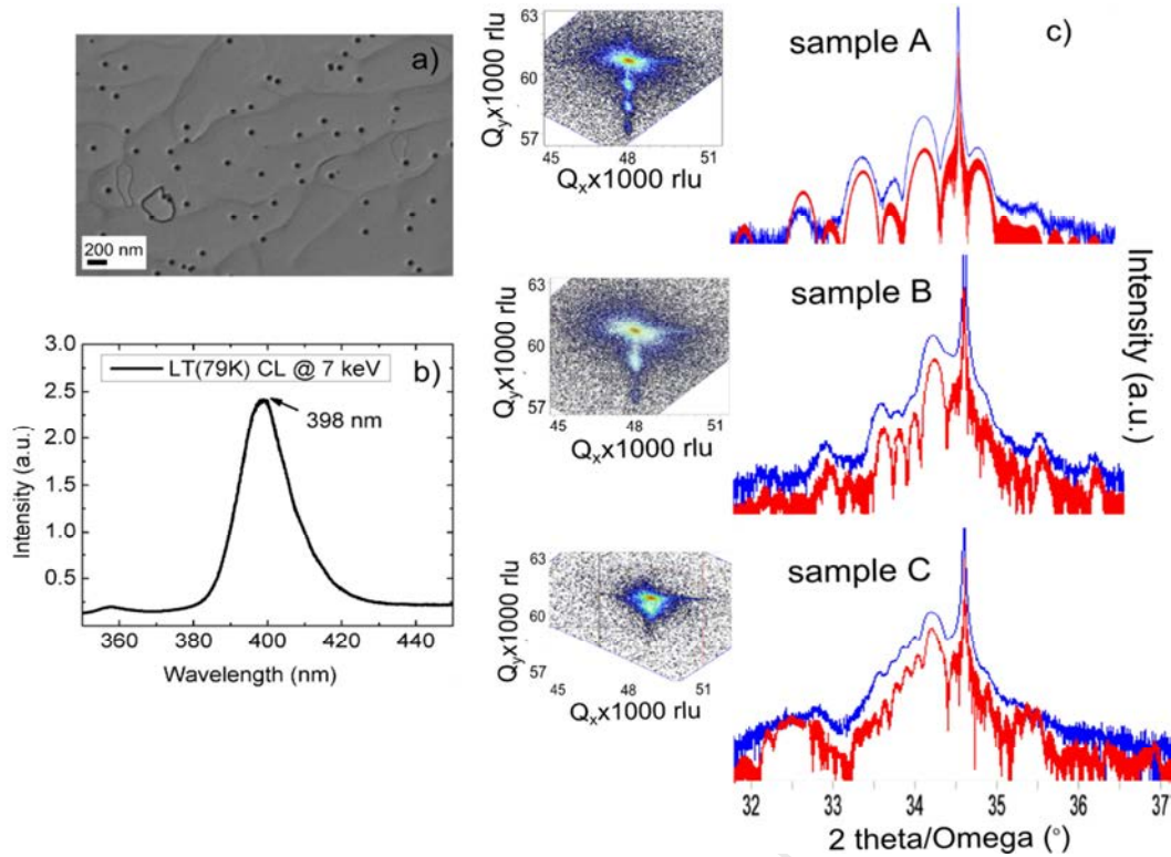
Fig. 2. SEM image of semi-bulk (SB) buffer sample (a), low temperature CL emission of SB buffer (b) and XRD 2\theta - \omega scan of sample A, B and C (c) (inset shows the RSMs).
