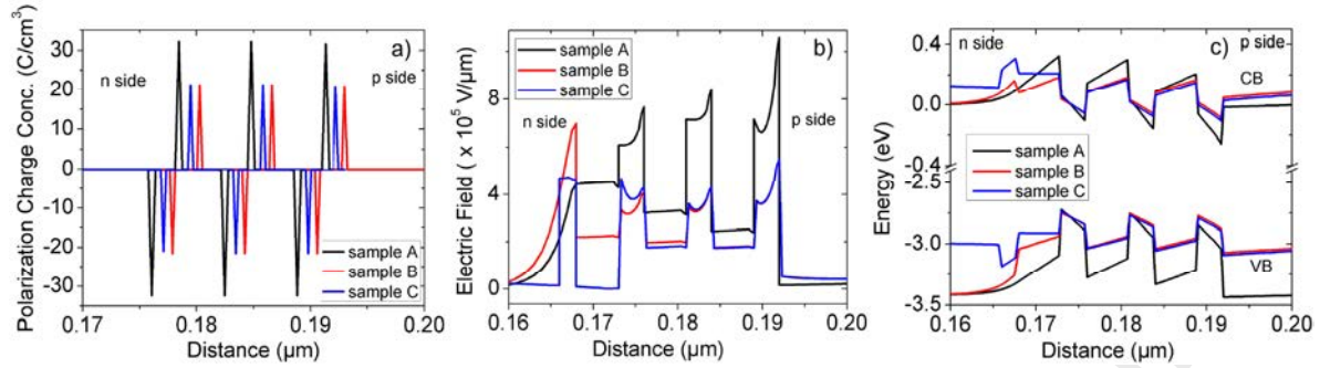
Fig. 4. Polarization charge concentration (a), internal electric field (b) and valence and conduction band structure (c) for the samples under study. Please note that, in (a), the distance scale has been shifted for sample A and B for better visibility.
