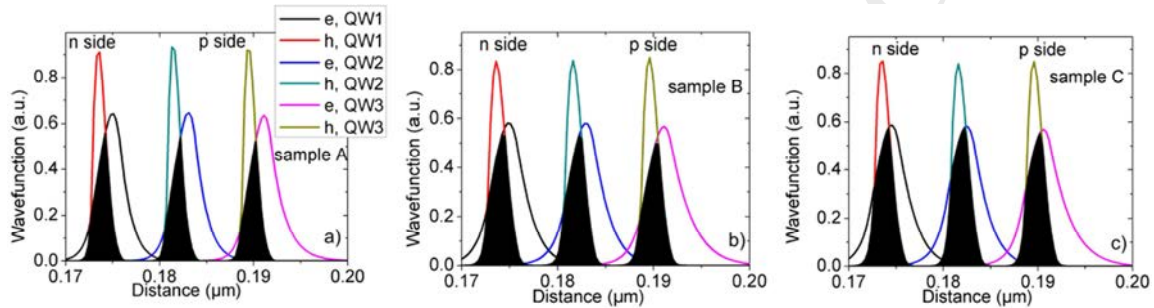
Fig. 5. Electron and hole wavefunction overlap for (a) reference sample A (b) reference sample B and (c) our final structure sample C.
