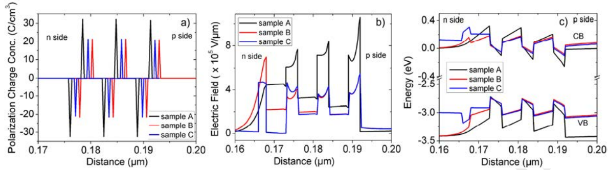
Fig. 4. Polarization charge concentration (a), internal electric field (b) and valence and conduction band structure (c) for the samples under study. Please note that, in (a), the distance scale has been shifted for sample A and B for better visibility.
