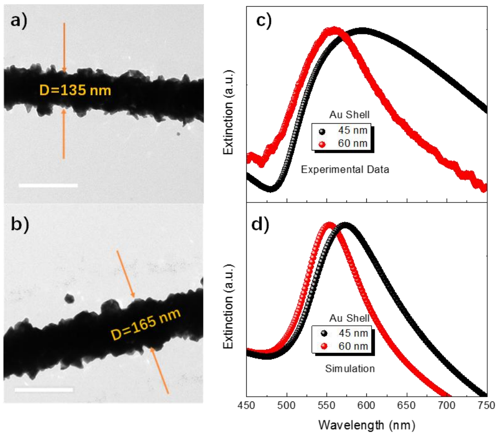
Figure 2. (a-b) Representatives TEM images of the nanoheterostructures and (c) experimental and (d) calculated extinction spectra of AgNWs/TiO 2 /GNS with 45 nm and 60 nm thickness of GNS. All scale bars: 200 nm.
