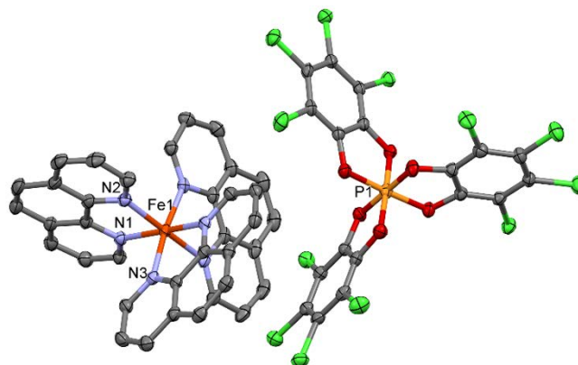
Figure 4. Complex [Fe(phen)_3](rac\text{-TRISPHAT})_2 ( 6 ) measured at 120 K. H atoms have been omitted for clarity, with displacement ellipsoids drawn at the 50% probability level.
