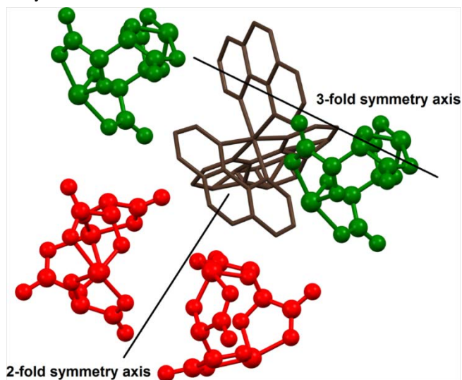
Figure 6. Interaction of the four closest [\Lambda\text{-As}_2(\text{tartrate})_2]^{2-} anions with [\Lambda\text{-Fe}(\text{phen})_3]^{2+} along 3- and 2-fold symmetry axes of complex 7 .
