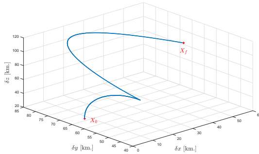
Fig. 7: Optimal 2-norm trajectory
