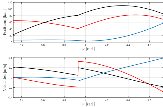
Fig. 5: Positions, velocities and cost in the 2-norm case
