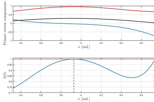
Fig. 6: Optimal primer vector in the 2-norm case
