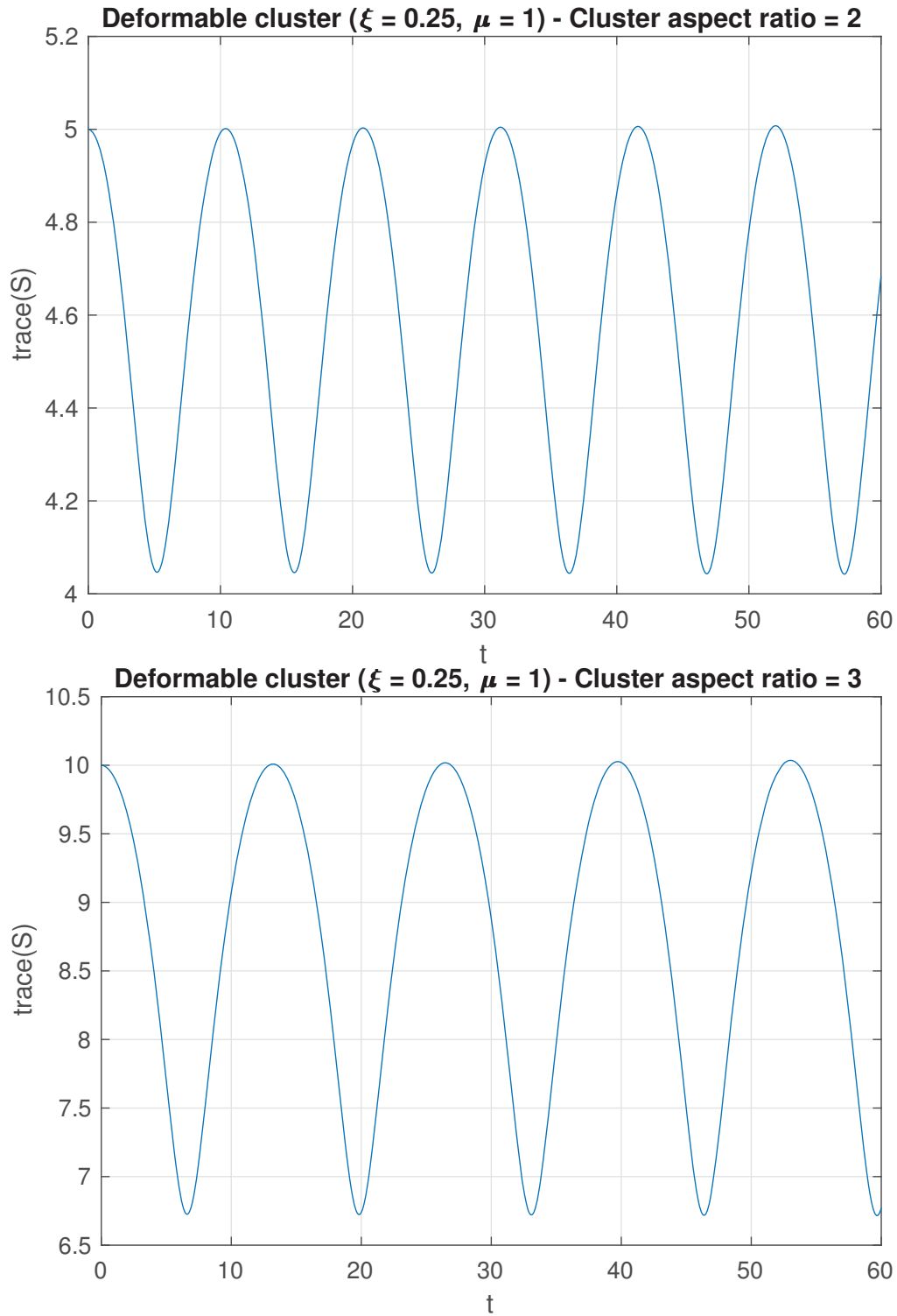
Fig. 5 Inertia tensor trace time evolution.
