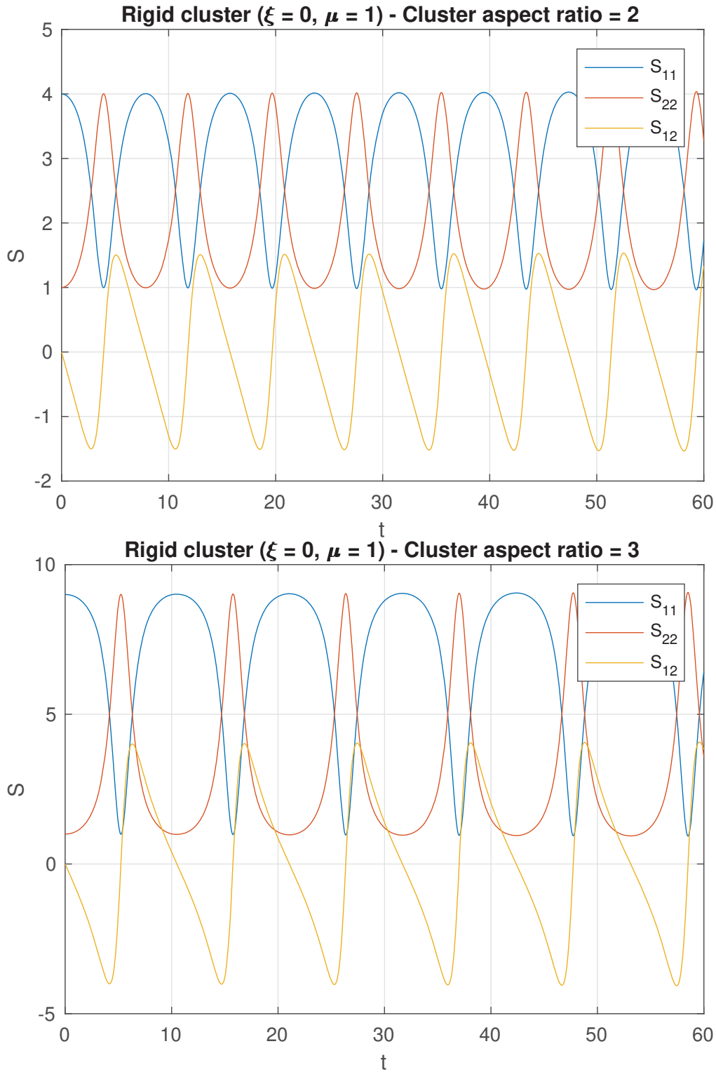
Fig. 3 Rigid clusters with different aspect ratio.
