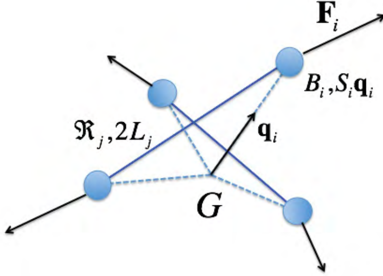
Fig. 1 Rigid cluster composed of rods.
