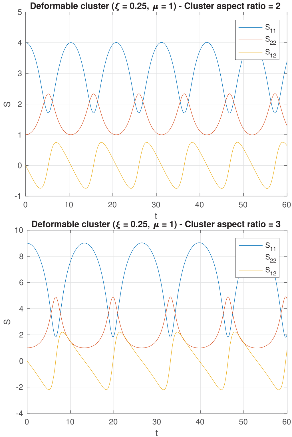
Fig. 4 Deformable clusters with different aspect ratio.
