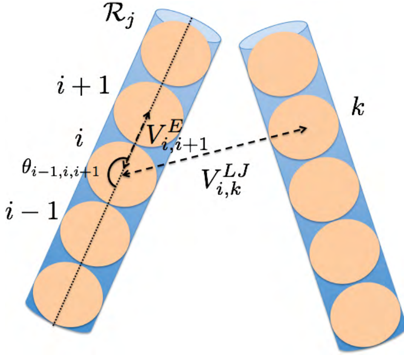
Fig. 2 Sketch of rods, particles and potentials
