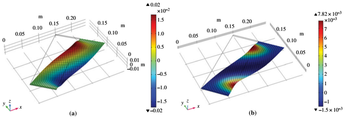
Fig. 24 Shear test. Qualitative buckled shapes of the first two bifurcation modes. Colors indicate values of the out-of-plane displacement. a First and b second buckling modes (color figure online)
