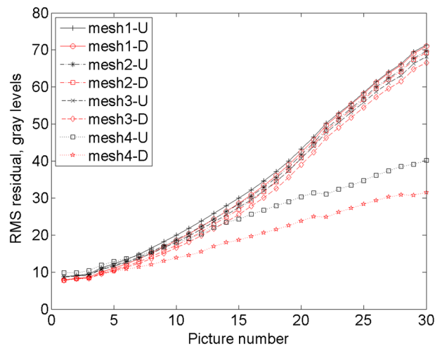
Fig. 40 RMS residual as a function of the picture number for the four meshes shown in Fig. 39. The extension U corresponds to updated registrations, and the extension D designates direct registrations
