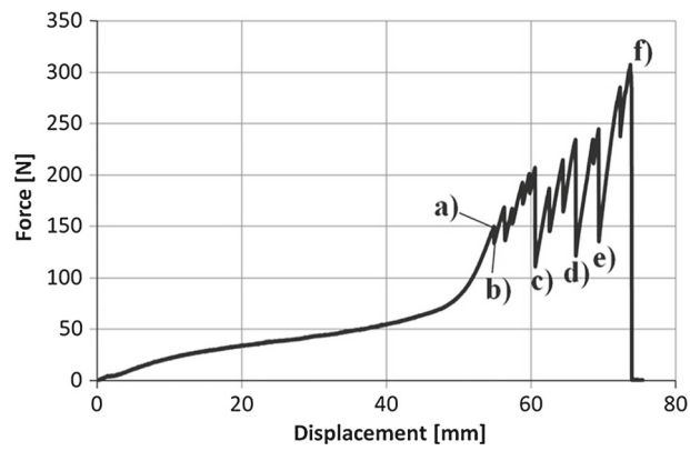
Fig. 31 Force versus prescribed displacement for a uniaxial bias extension test. a Sample before first beam breakage (i.e., breakdown onset); b upper-left corner beam breakage; c–f further fiber breakage
