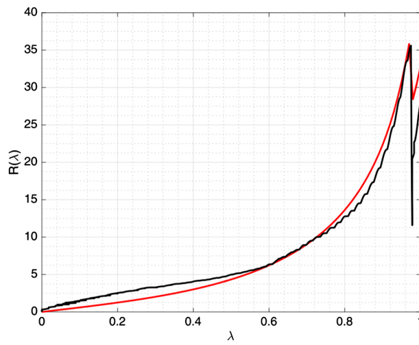
Fig. 34 Force ( N ) versus non-dimensional displacement for the shear test of a pantographic sheet up to the onset of fiber rupture. The black curve is the experimental data, and the red curve has been obtained via numerical simulation (color figure online)
