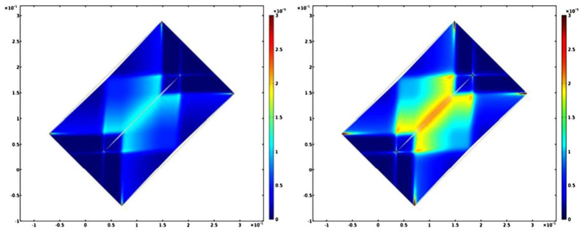
Fig. 26 Effect of a cut inside a sheet. Eulerian representation of the elastically stored energy density for a sheet with lower shear stiffness (left) and for a sheet with higher shear stiffness (right), both subject to a standard bias extension test
