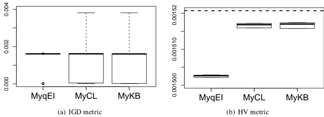
Figure 5: Boxplots of the metrics computed for the three best methods over 100 simulations for the six-hump Camel function with derivative observations.
