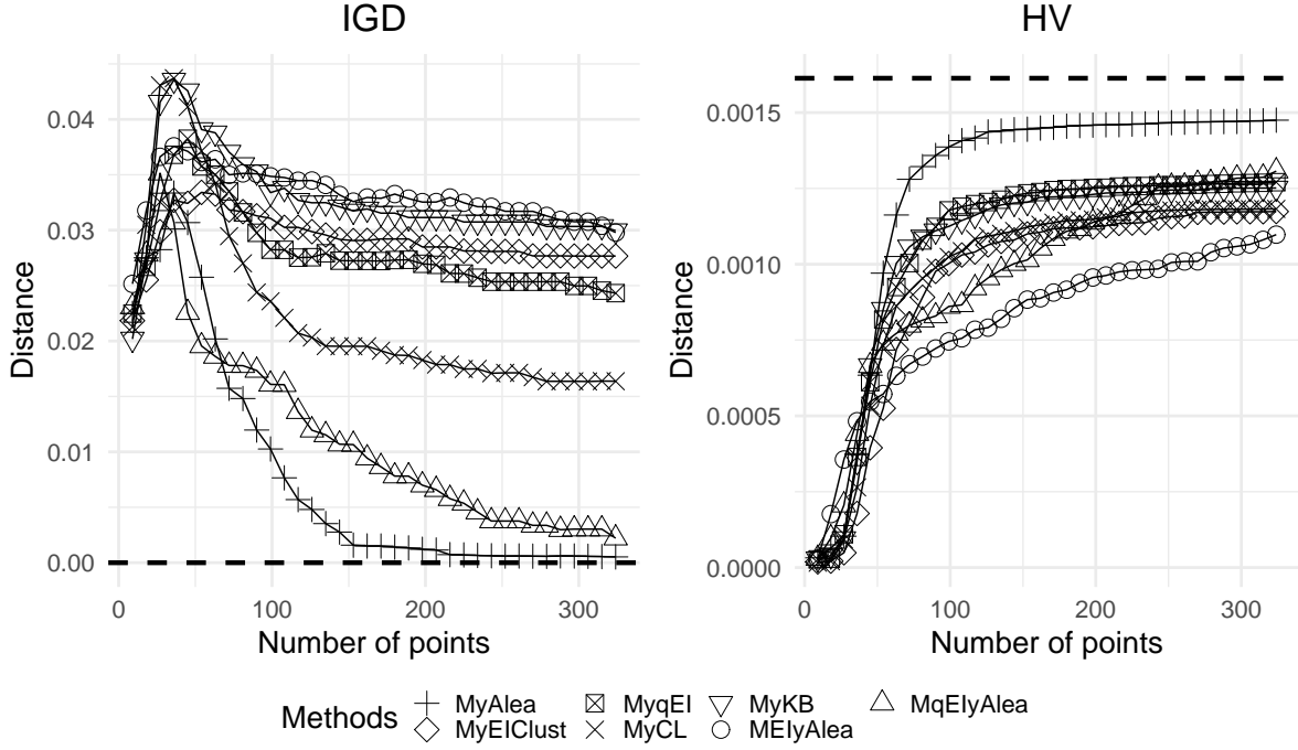
Figure 6: Six-hump Camel function without derivatives' observations. Evolution of the Pareto metrics with the number of points compute for all the methods over 100 different runs of the algorithm. The HV value of the theoretical front is represented by the dotted line.
