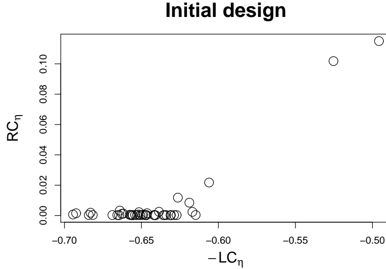
Figure 10: The 46 initial observation points in the true objective space: opposite level criterion ( -LC_\eta ) and robustness criterion calculated on the efficiency ( RC_\eta ).
