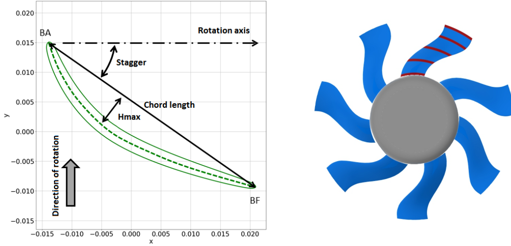
Figure 9: Blade section with the three input parameters on the left. Sections are represented on the right by the red lines along one blade. Section 1 is the closest to the disc and section 5 the most far away.
