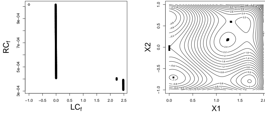
Figure 3: Pareto front of the six-hump Camel function in the objective space (left) and in the parameter space (right).
