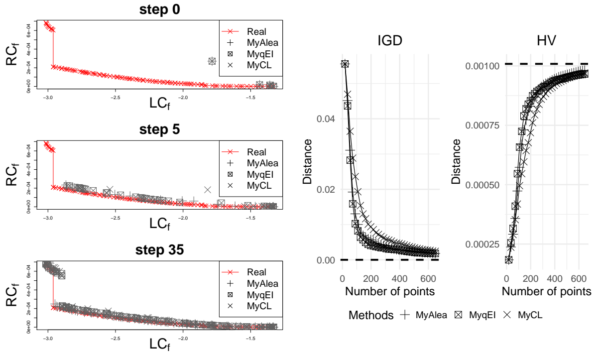
Figure 8: On the left: Pareto fronts obtained during the optimization procedure of the three strategies at the initial step (step 0), step 5 and final step (step 35). On the right: evolution of the metrics during the algorithm computed for all the methods in 100 simulations for the Hartmann function with no derivative observation. The HV value of the theoretical front is represented by the dotted line.
