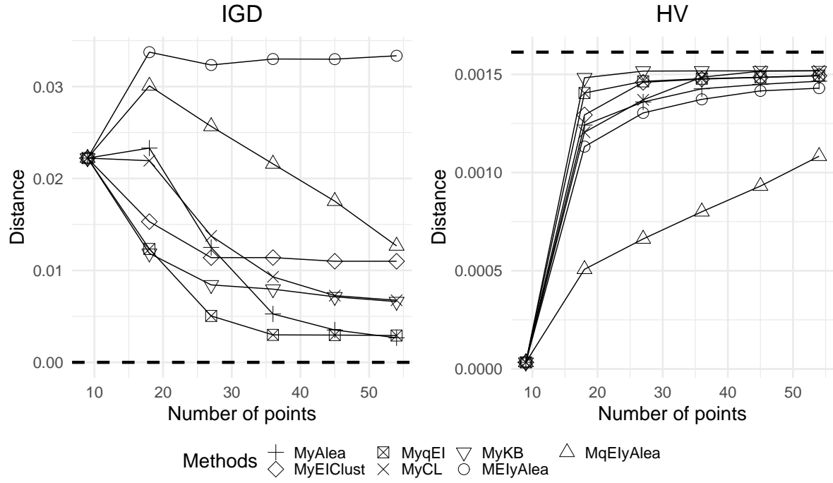
Figure 4: Six-hump Camel function with derivative observations. Evolution of the Pareto metrics with the number of points computed for all the methods over 100 different runs of the algorithm. The HV value of the theoretical front is represented by the dotted line.
