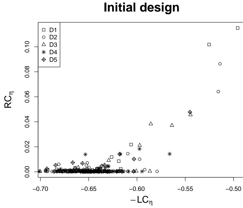
Figure 14: The initial observation points for five LHS designs in the true objective space: opposite level criterion ( -LC_{\eta} ) and robustness criterion calculated on the efficiency ( RC_{\eta} ).
