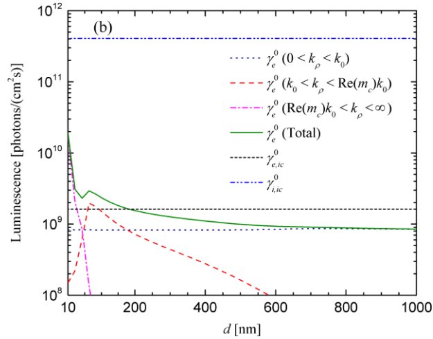
FIG. 3. Cell external luminescence in chemical equilibrium ( \gamma_e^0 ) as a function of the gap thickness ( d ) for t = 10 \mu\text{m} : (a) Si emitter. (b) Drude emitter. For comparison, internal luminescence ( \gamma_{i,ic}^0 ) and external luminescence ( \gamma_{e,ic}^0 ) of an isolated cell are also plotted.
