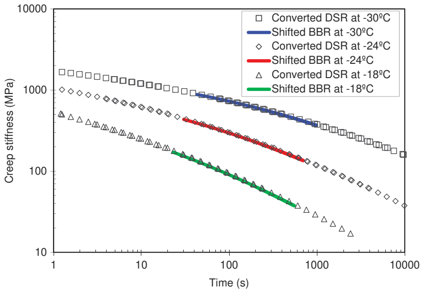
Figure 10. Creep stiffness for AAD1, shifted BBR and converted DSR data.
