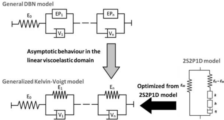
Figure 6. Analogical 1D representation of the DBN model, which corresponds to the GKV model in the LVE domain (small strain amplitude).
