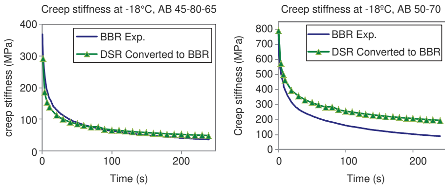
Figure 9. Comparison of DSR and BBR data for the German asphalt binders at -18^{\circ}\text{C} .
