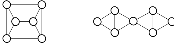
Figure 2: G_6 and G_7 two minimal expandable graphs with 6 and 7 vertices.
