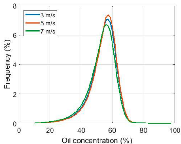
Figure 15. Normalized histograms of oil concentration estimated within the mineral oil slick released during the MOS Sweeper exercise (10:02 UTC) for an input wind speed of 3 m/s (blue), 5 m/s (red) and 7 m/s (green).
