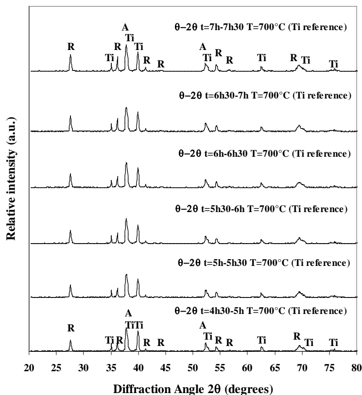
Figure 6. In-situ high-temperature XRD experimental diffractograms performed on titanium bulk reference sample annealed at T = 700^\circ\text{C} in air (Ti: titanium, A: anatase, R: rutile) from 4 h 30 to 7 h 30.
