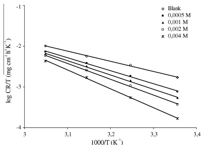
Figure 5 Transition-state plots for carbon steel corrosion rates (CR) in 1 M HCl with and without different concentrations of HMDTMPA acid.
