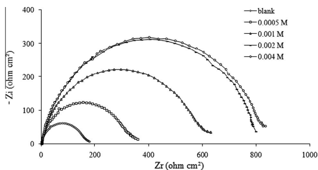
Figure 8 Nyquist plot for HMDTMPA in 1 M HCl with and without different concentrations of HMDTMPA.
