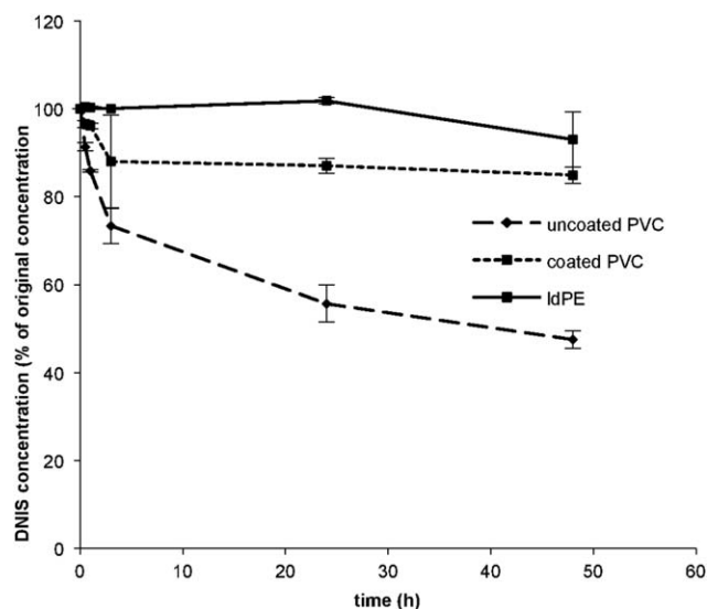
Figure 9. Remaining concentrations of DNIS after contact with uncoated PVC ( n = 15 ), coated PVC ( n = 15 ), and IdPE ( n = 15 ).
