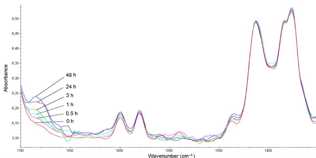
Figure 10. FTIR-ATR spectrum performed between 1700\text{ cm}^{-1} and 1400\text{ cm}^{-1} on uncoated PVC in contact with diazepam. [Color figure can be viewed in the online issue, which is available at wileyonlinelibrary.com .]
