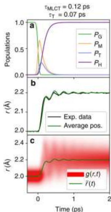
Figure 5. Simulations of the transient molecular distribution in coordinate r for MLCT \rightarrow HS ( \tau_{\text{MLCT}}=120 fs) and MLCT \rightarrow ^3\text{T}\rightarrow HS ( \tau_{\text{T}}=70 fs) electronic state transition (a–c,d–f, respectively). The time-dependent populations of the different electronic states are shown in panels (a and d), which give rise to the calculated distribution g(r,t) and average coordinate r \bar{r}(t) (c,f). The experimental data at 7145 eV (blue) scaled in r has additionally been overlaid with the simulated signal (b,e). Reprinted with permission from NPG [1b] .
