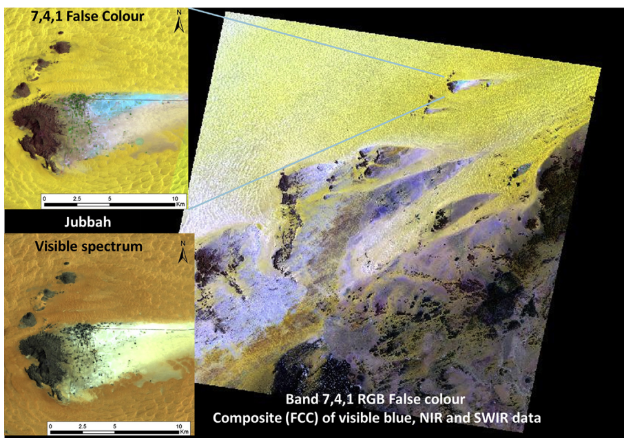
Fig. 5. Example of 7,4,1 TM FCC's for visual discrimination of initial palaeolake deposits for use as spectral training sites for the large known palaeolake basin of Jubbah. Note that although the basin appears uniformly white (high reflectance) across the visible spectrum, palaeolake deposits (primarily deflated gypsiferous deposits in this instance) can be readily differentiated in blue tones in the multispectral FCC data. (For interpretation of the references to colour in this figure legend, the reader is referred to the web version of this article.)
