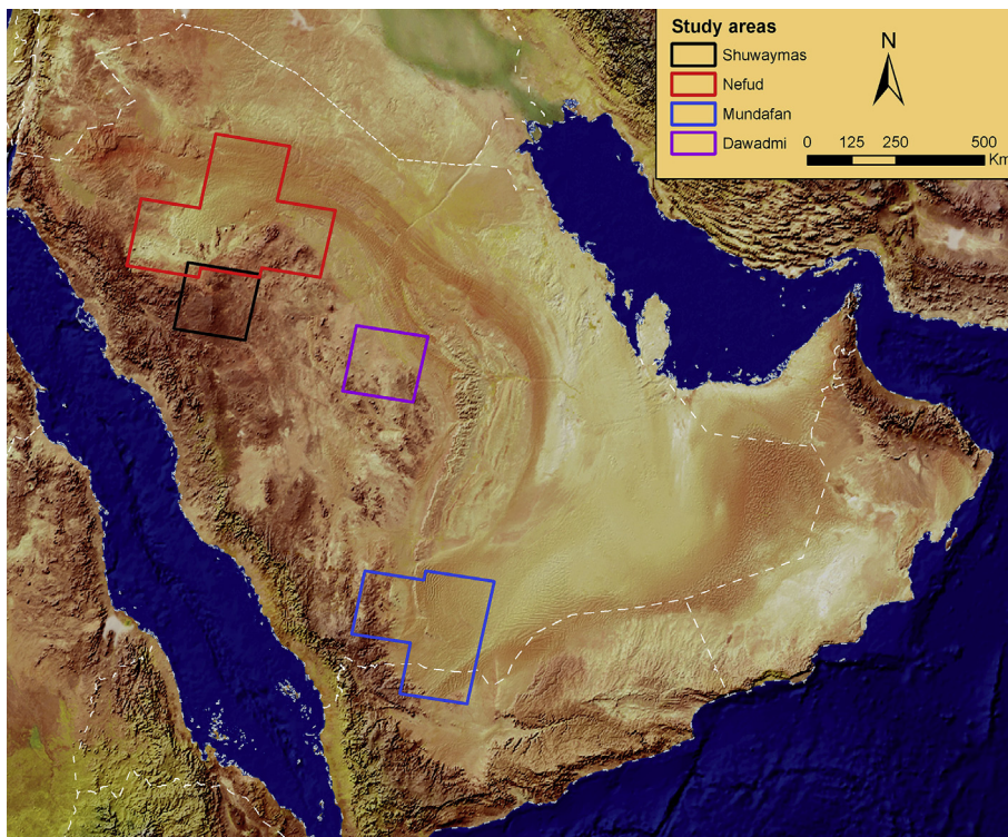
Fig. 4. Location of initial study regions discussed in this paper and used as test bed areas for the defined method, overlain on Natural Earth 2 basemap, with international borders marked. Note that the Shuwaymas and Nefud regions are treated collectively in Figs. 6, 11 and 12, due to their proximity.
