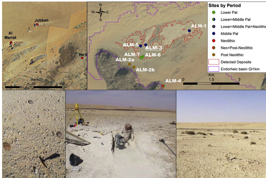
Fig. 9. The Al Marrat basin and materials identified by the classifier. Clockwise from top left; regional location; deposits identified by the classifier within the basin and archaeological site locations; detected gypcrete mesas; Excavation at the ALM-3 stratified site (see Jennings et al. forthcoming); and Acheulean surface scatter.
