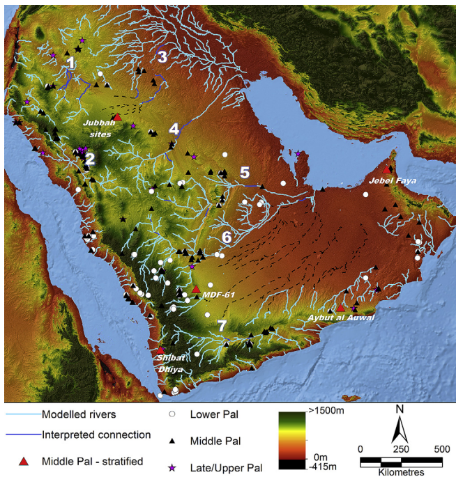
Fig. 10. Principal modelled palaeodrainage of the peninsula (>1000 km 2 contributing area, strahler stream order 2 and above, pruned for clarity-see Fig. 2 for unpruned data), with interpreted Pleistocene connections (early and late) reinstated and published archaeological site locations. Stratified dated sites are labelled. Major drainage systems: 1; Wadi Sirhan trough, 2; Wadi al Hamd, 3; Euphrates (note that due to this region still receiving runoff drainage in the central Euphrates-Tigris depression may reflect recent activity, and should be considered indicative only), 4; Wadi ar Rimah/Batin, 5; Wadi Sabha, 6; Wadi ad Dawasir, 7; Wadi Hadramawt. Drainage in dunes differentiated (dashed lines).
