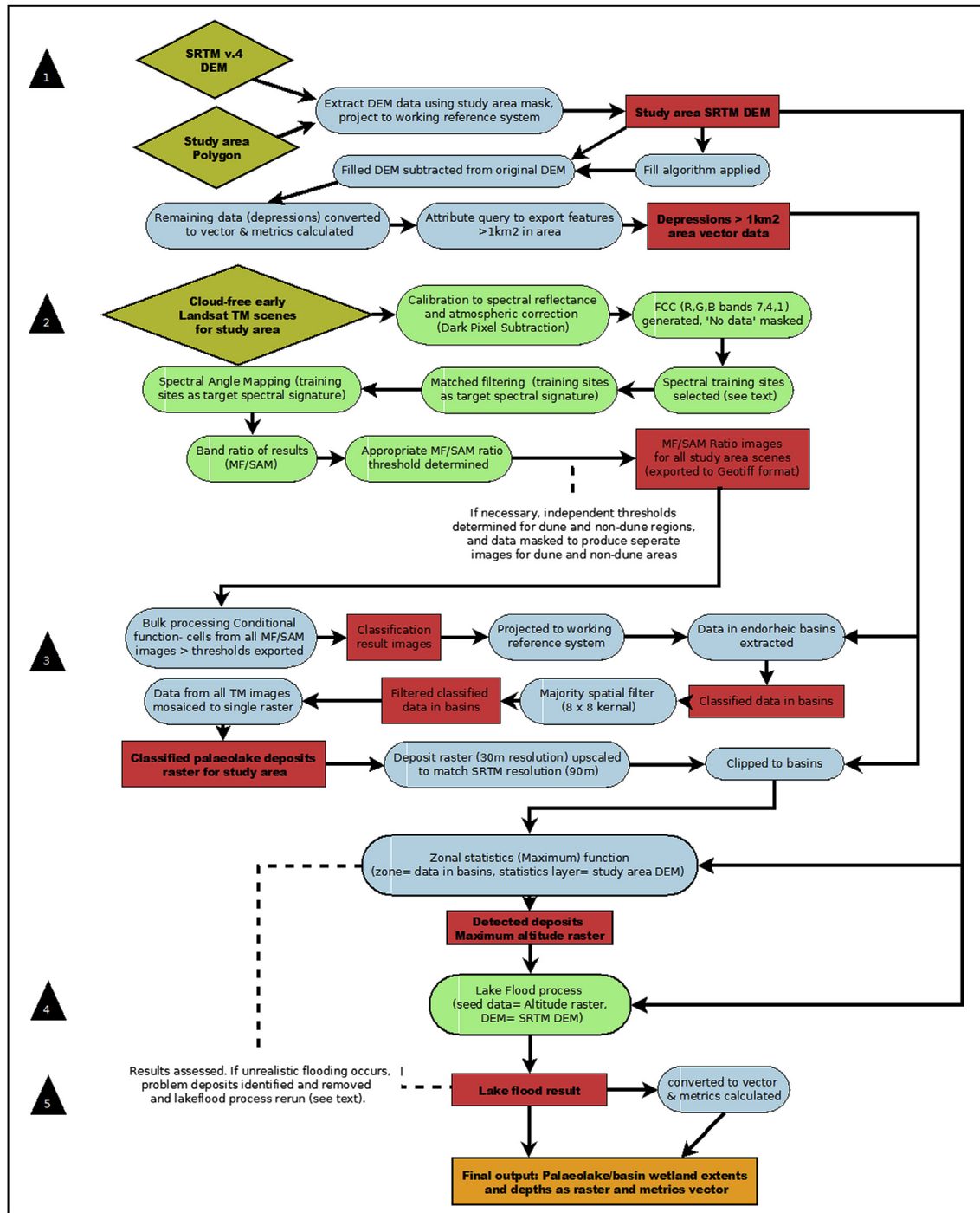
Fig. 3. Our palaeolake mapping GIS workflow (simplified schematic). Required initial input data is shown in diamonds. Processing steps are in rounded boxes. Output datasets resulting from processing are in red square boxes, with prominent outputs in bold. Stages 1, 3 & 5 (blue) are performed in ESRI ArcGIS and have been automated as custom tools. Stages 2 and 4 (green) are performed manually in ENVI and SAGA GIS, respectively. (For interpretation of the references to colour in this figure legend, the reader is referred to the web version of this article.)
