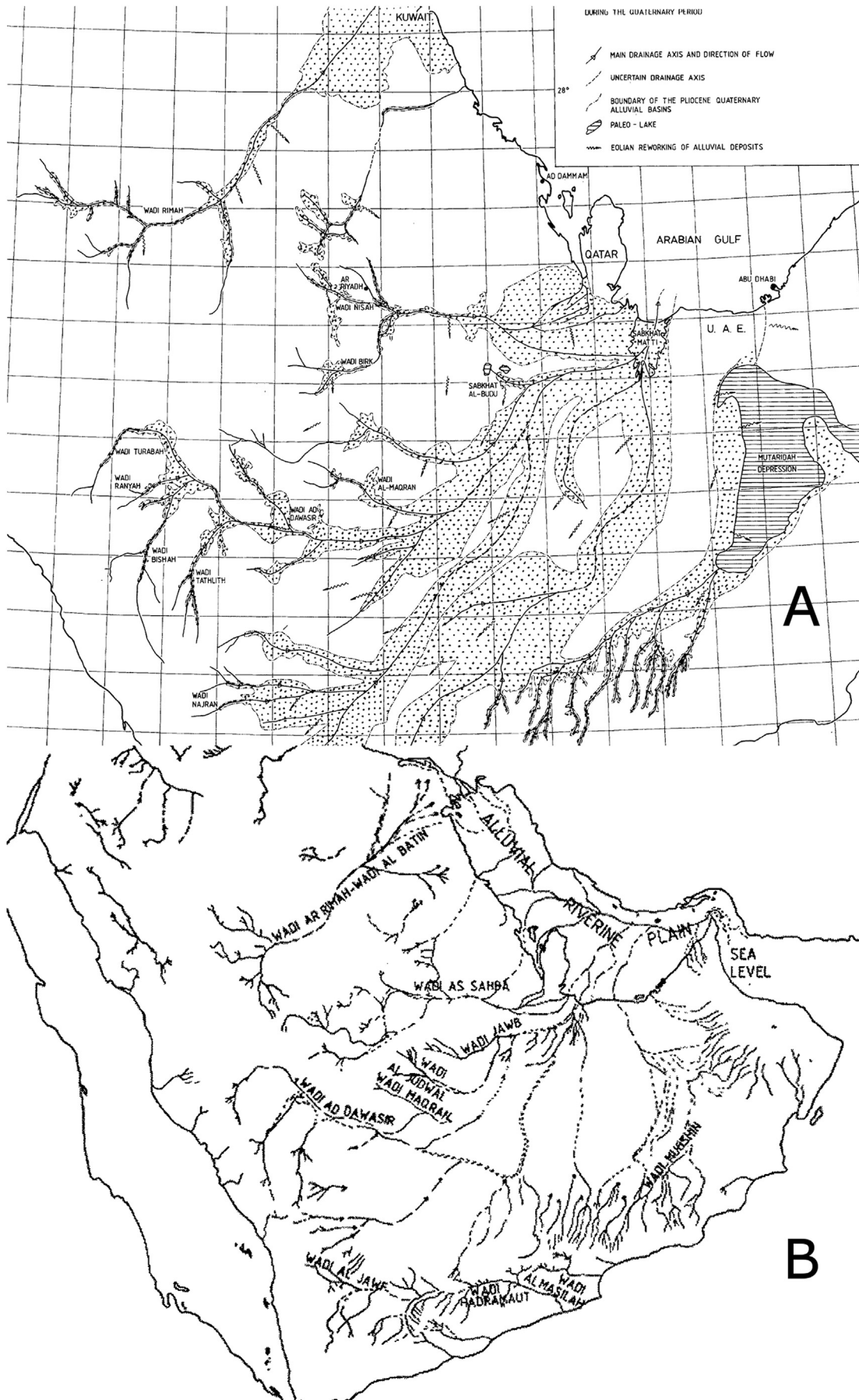
Fig. 1. Prior overview peninsula-scale maps of principal palaeodrainage systems for (A) the early Quaternary (Anton, 1984) and (B) the Late Pleistocene (Edgell, 2006). Both images reproduced with kind permission from Springer Science and Business Media.
