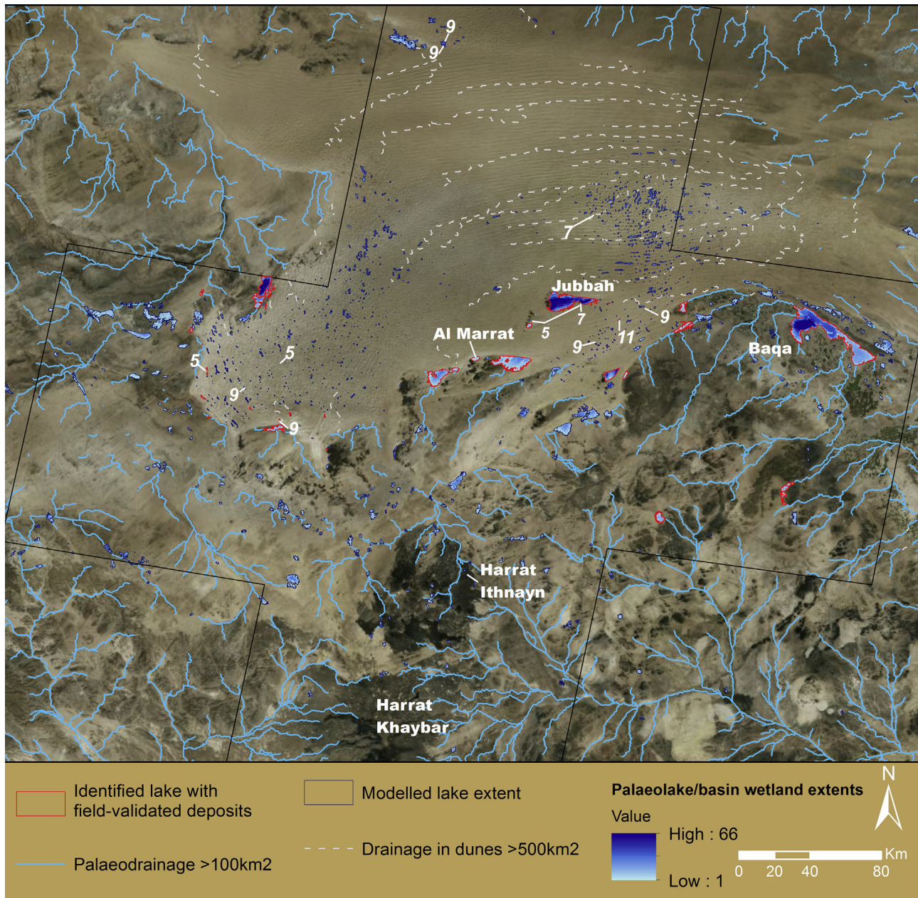
Fig. 12. Modelled palaeohydrology for the Nefud and Shuwaymas study areas displayed over Bing Maps imagery. Locations discussed in the text are labelled, and modelled lakes containing deposits that have been field validated as lake deposits are marked in red. Numbers show the MIS phase of formerly dated lake locations (Petraglia et al., 2011, 2012; Rosenberg et al., 2013) also mapped by our method. (For interpretation of the references to colour in this figure legend, the reader is referred to the web version of this article.)
