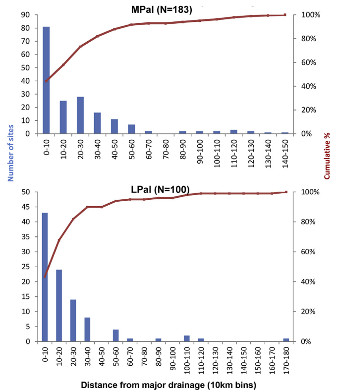
Fig. 11. Histograms of distance from the principal modelled palaeodrainage displayed in Fig. 10, for Middle and Lower Palaeolithic sites from Groucutt and Petraglia (2012). Only distance to the largest major drainage systems has been assessed, to provide a conservative assessment.
