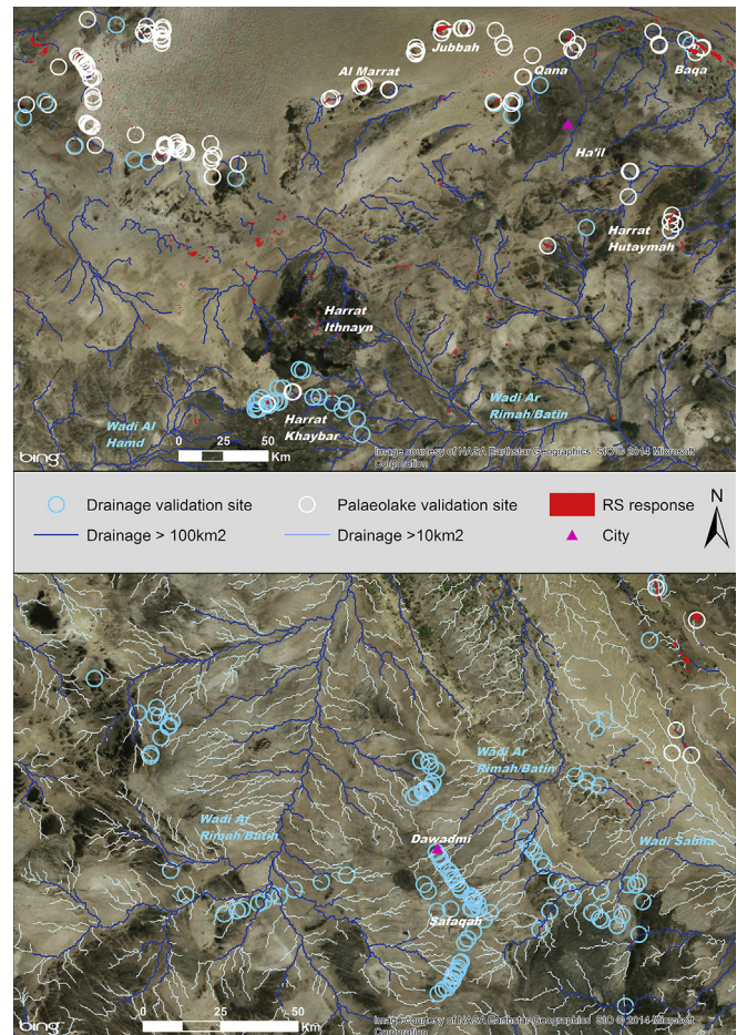
Fig. 6. Field validation locations in the Nefud & Shuwaymas (top) and Dawadmi (bottom) regions, for potential identified palaeolake deposits (final deposits from workflow displayed in red, exaggerated for visibility), and modelled drainage. Questionable drainage modelled in dunes not displayed for clarity (see text). Base imagery is Bing maps, with key geographic locations and features discussed in the text labelled. (For interpretation of the references to colour in this figure legend, the reader is referred to the web version of this article.)
