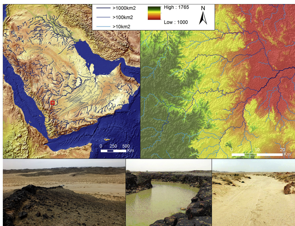
Fig. 2. Examples of scaling of drainage data, and of field validated drainage courses. Upper left, >1000 km 2 major drainage courses in dark blue (questionable drainage in dunes in grey, and no interpreted former connections displayed), with location of detail area (upper right) marked in red, overlying Natural Earth 2 basemap. Detail map (upper right) shows drainage data of varying catchment area scales, illustrating how as catchment area threshold is lowered, progressively smaller tributaries of drainage systems are plotted. Lower images show examples of field validated mapped drainage courses from the Dawadmi and Shuwaymas regions. Centre image is the location of the SH-11 site with ponded standing water (see text and Groucutt et al., 2015), whilst the lower right image shows minor headwaters (<10 km 2 catchment) with associated Acheulean archaeology near Safaqaq (Jennings et al., 2015). (For interpretation of the references to colour in this figure legend, the reader is referred to the web version of this article.)
