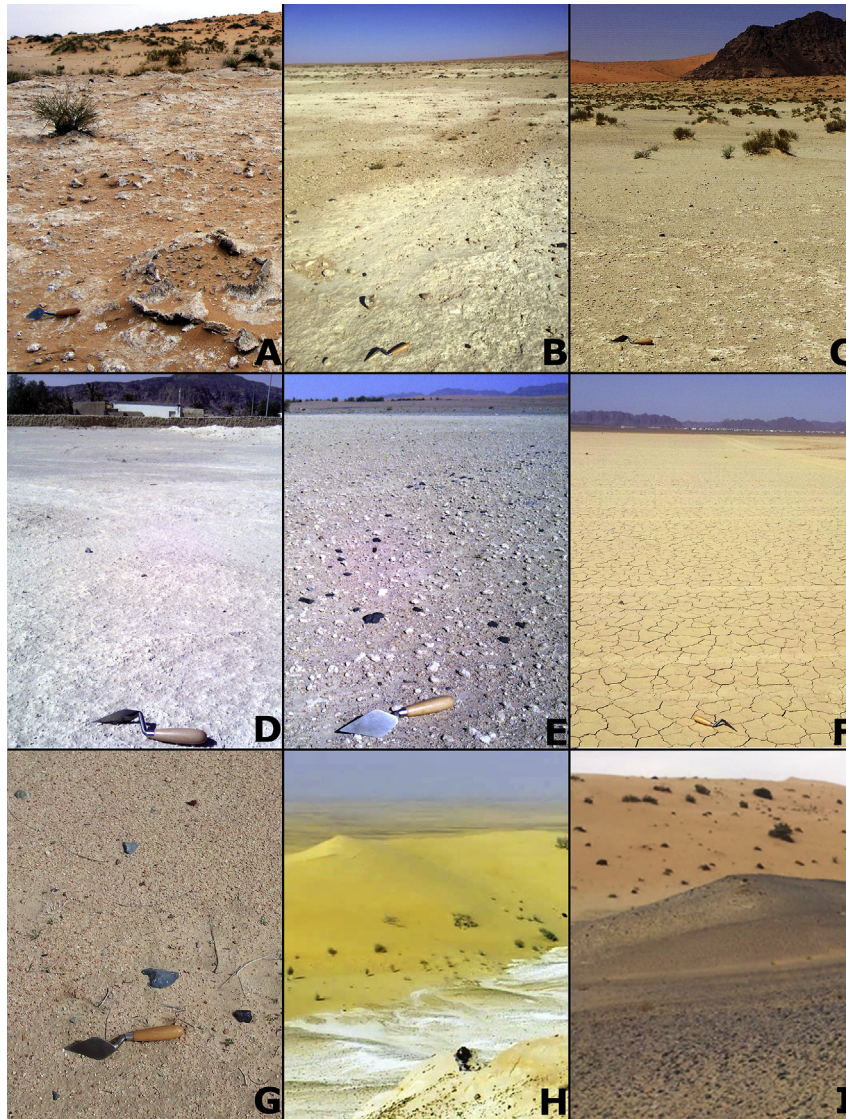
Fig. 8. Typical examples of surface characteristics of field tested sites from the Nefud study area. A: Interdunal gypcrete with dessication curls capping lacustrine silts, Jubbah basin. B: Marl, Khabb Araf basin. C: Gypcrete, Khabb Araf basin D: Reworked gypsiferous and carbonate rich sediments, Jubbah basin. E: Calcrete, Hufayr basin. F: Khabra' playa pan, Harrat Hutaymah. G: Incipient palaeosol with Middle Palaeolithic tools, (QAN-1 site) H: Bleached palaeodune (fore and mid-ground) western Nefud. I: Heavily indurated gypcrete/marl (western Nefud).
