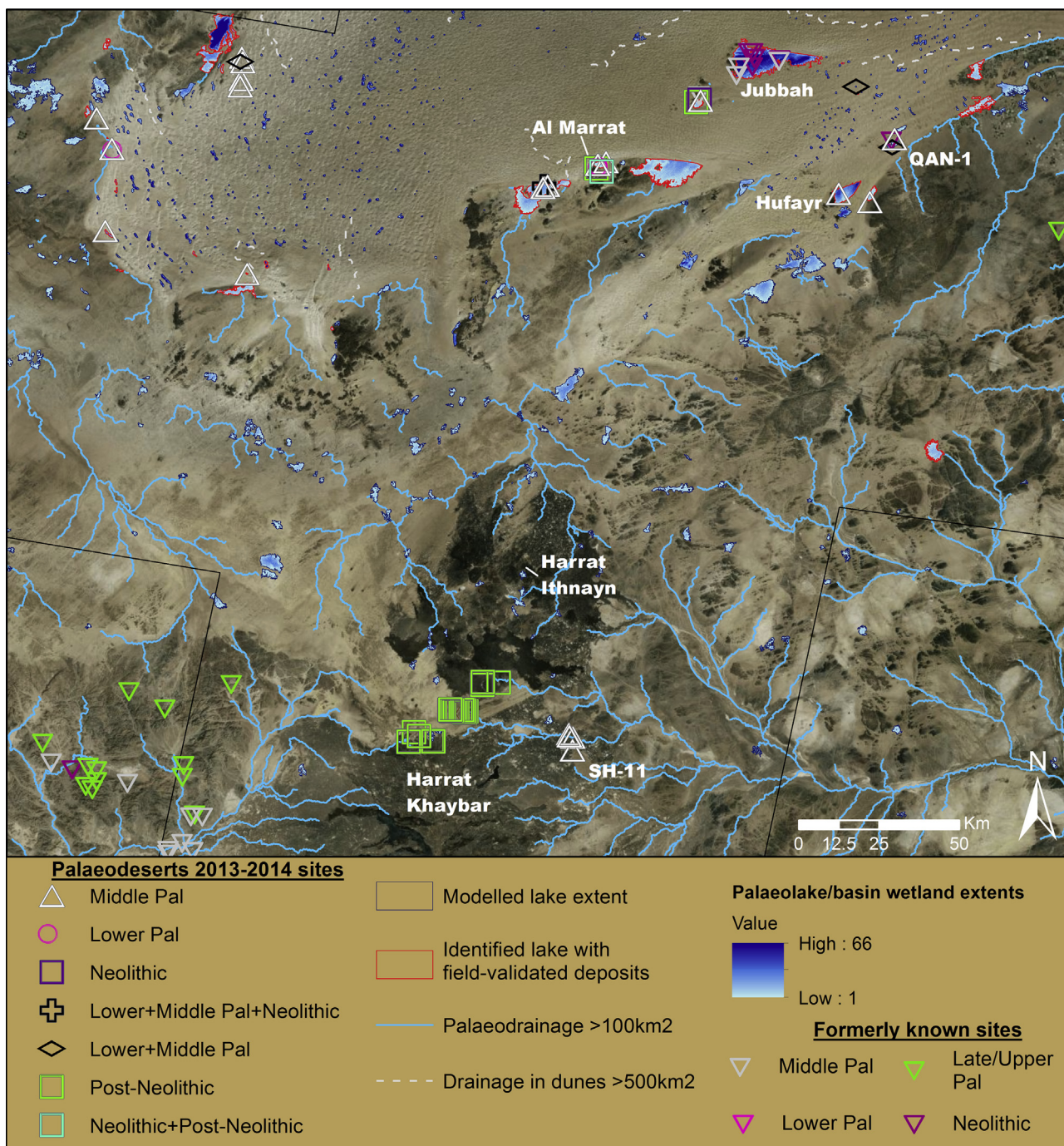
Fig. 13. Archaeological sites identified during palaeohydrologically targeted survey within the Nefud and Shuwaymas study areas, differentiated by period and displayed over Bing Maps imagery and palaeohydrological data. Sites and locations discussed in the text are labelled.
