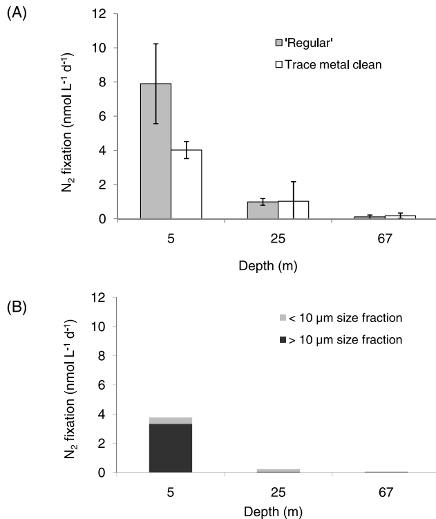
Figure 4. (a) Nitrogen fixation rates measured at station 25 at three depths, using both trace metal clean conditions (white bars) and non-trace-metal clean (“regular”) conditions (gray bars). The error bars represent the standard deviation on the triplicate measurements. (b) Nitrogen fixation attributed to the >10-μm fraction (dark gray) and the <10-μm fraction (light gray). The size fractionation had been performed under trace metal clean conditions.
