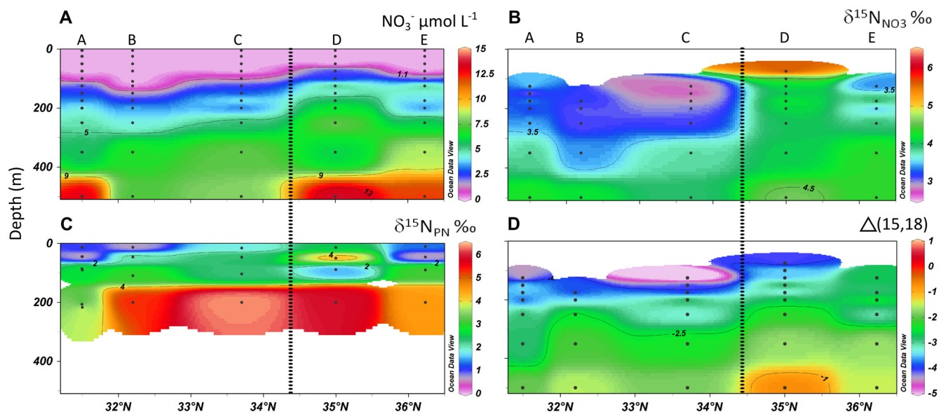
Fig 4. Geochemical tracers of N 2 -fixation along the DIAPICNA cruise transect. Longitudinal cross-sections of (A) nitrate concentration, (B) \delta^{15}\text{N}_{\text{NO}_3} signal, (C) PN isotopic signature and (D) \Delta(15,18) —see eq (2) . The position of the Azores Front is indicated by a dashed line, and station i.d. is given on top.
