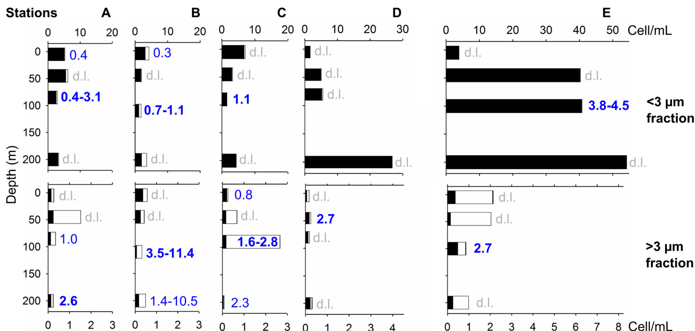
Fig 7. N 2 -fixation rates and UCYN abundance in <3 μm and >3 μm particles. Top panels: <3 μm particles; bottom panels: >3 μm particles. For each station and depth, N 2 -fixation rates ( \mu\text{mol m}^{-3} \text{d}^{-1} ) measured in each size fraction are indicated in blue (d.l. indicate measurements below the detection limit). Black bars indicate free pico-UCYN, white bars for associated pico-UCYN and grey bars for large pico- or nano-UCYN (in \text{cell mL}^{-1} ).
