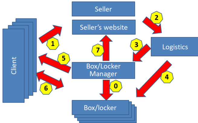
Fig. 2. Software architecture with main modules and exchanges.
