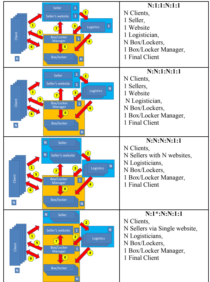
Fig. 3. Different working configurations.
