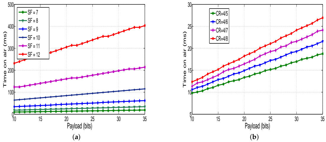
Figure 8. (a) Time on air vs. payload at different SF; and (b) time on air vs. payload at different CR.
