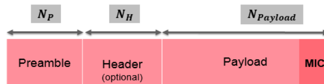
Figure 6. LoRa ACK structure.
