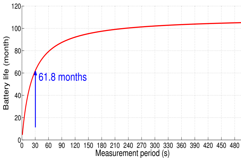
Figure 16. Sensor node autonomy: Scenario 1.
