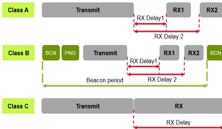
Figure 4. Different LoRaWAN classes.
