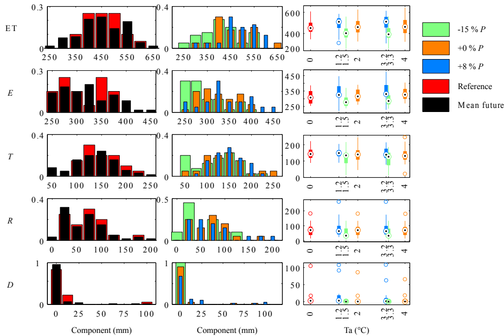
Figure 2. Simulation results for the annual components of the water cycle (Top to Down: ET , E , T , R and D ). Left: frequency histograms for reference (Sc0) and scenario-averaged future climatic scenarios (Sc1–Sc6). Middle: frequency histograms for the three precipitation periods. Right: boxplots of annual components of the water cycle as a function of temperature scenarios. Water cycle components correspond to x axis in the left and middle columns, and to y axis in the right column.
