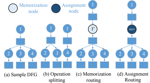
Figure 8: Graph transformation
