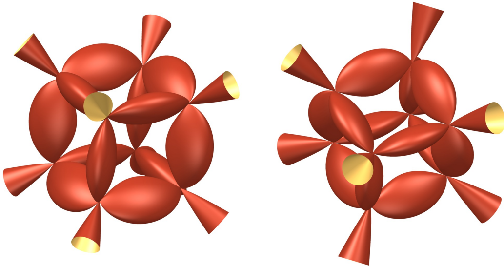
FIGURE I. Part of the real locus of \mathcal{Z}(F_{u_3}) for W = G_{29} .
