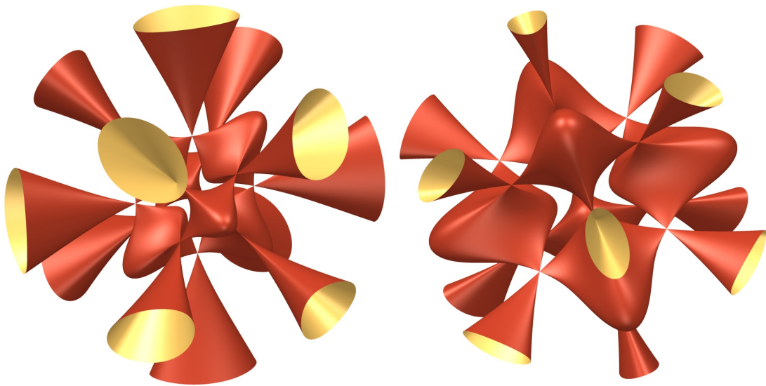
FIGURE II. Part of the real locus of \mathcal{Z}(F_{u_1, v_1}) for W = G_{29} .
