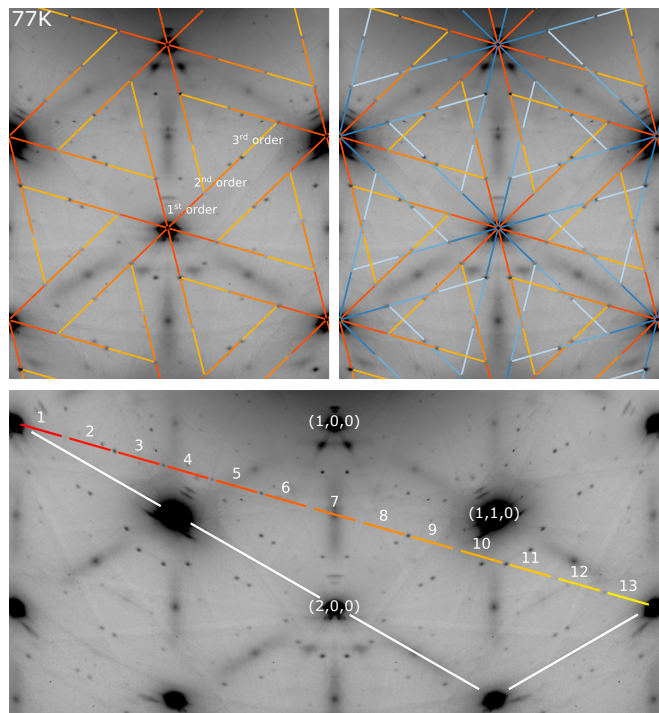
FIG. 4. Two interwoven commensurate superlattices. Diffuse scattering of 2H-NbS 2 in the (h, k, 0) plane at 77 K. The ring of 12 satellite peaks around each Bragg peak, and the four peaks around the M point can be indexed with two wave vectors. (Upper left panel) Subset of peaks indexed by \vec{q}_1 = \frac{3}{13} \vec{a}^* + \frac{1}{13} \vec{b}^* , with first, second, and third order reflections. (Upper right panel) Both subsets of peaks indexed by \vec{q}_1 in shades of red, and its mirror image \vec{q}_2 = \frac{4}{13} \vec{a}^* - \frac{1}{13} \vec{b}^* in shades of blue. (Lower panel) \vec{q}_1 and \vec{q}_2 are commensurate with the crystal lattice via 13 \vec{q}_1 = 3 \vec{a}^* + \vec{b}^* . The wave vectors length is ||\vec{q}_{1,2}|| = \frac{1}{\sqrt{13}} ||\vec{a}^*|| so that each defines a \sqrt{13} a \times \sqrt{13} a superlattice in real space. This is also geometrically equivalent to 3\vec{q}_1 - \vec{q}_1' = \vec{a}^* , where \vec{q}_1' is \vec{q}_1 rotated by +120^\circ , which clearly appears in the upper panels. Note that the upper panels show the same region as in Fig. 2, and that the lower panel is an extended view centered on this same region.
