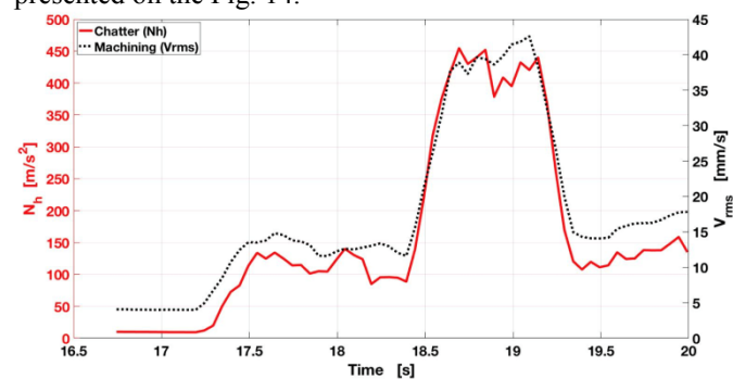
Fig. 14. Test of chatter detection (setup – 4)
