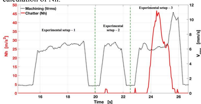
Fig. 13. Test of chatter detection for different setups
