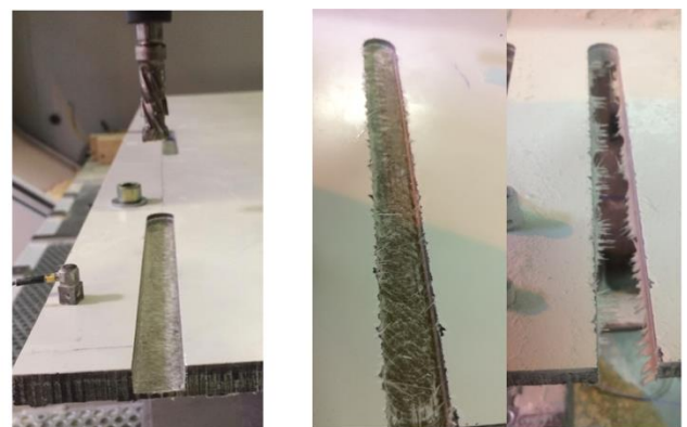
a) The path with new tool (type of the tool condition - 1) b) The path with damaged tool (type of the tool condition - 4)
