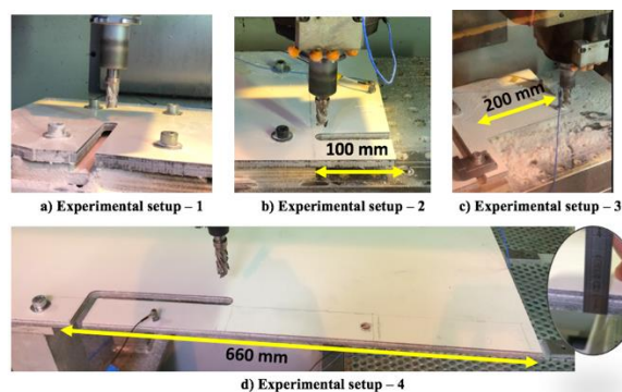
Fig. 3. Experimental setups
