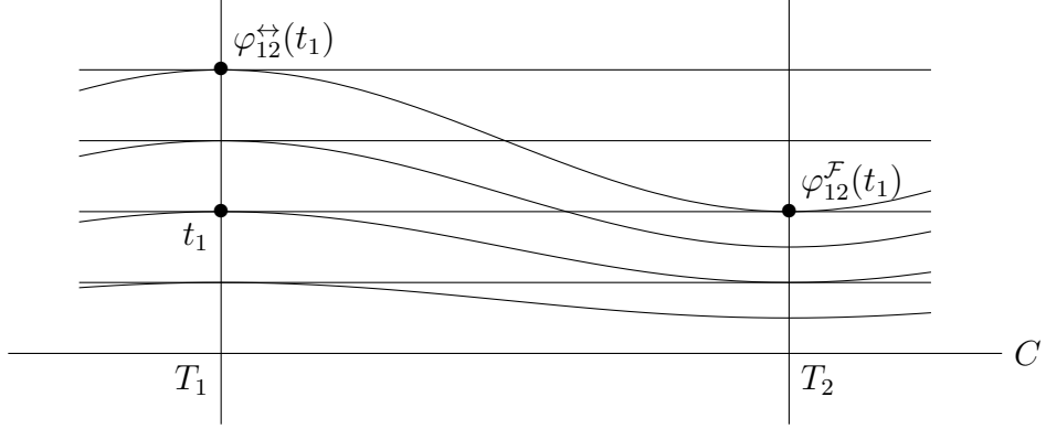
Figure 4: Holonomy transports
