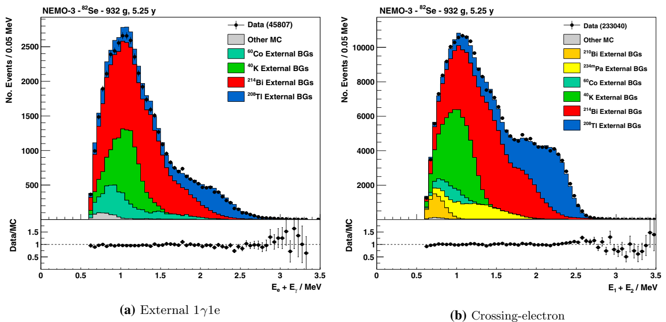
Fig. 2 a Distribution of the sum of the energies of the electron and \gamma -ray in the external 1\gamma 1e channel. b Distribution of the sum of the incoming and outgoing electron energies in the crossing-electron channel. In both figures, the energy spectra from data are compared to the
