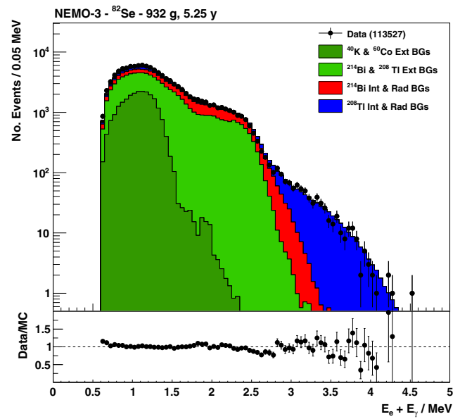
(b) 1e1 \gamma Channel
