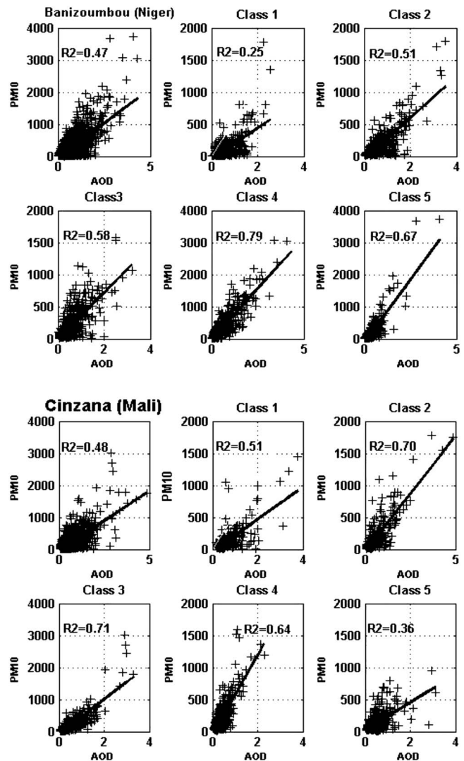
Figure 12. Relationship between the observed particulate matters (PM 10 ) Obs (µg/m 3 ) and the AOD for the whole studied period (upper left cartoon) and for each weather type at the two stations.
