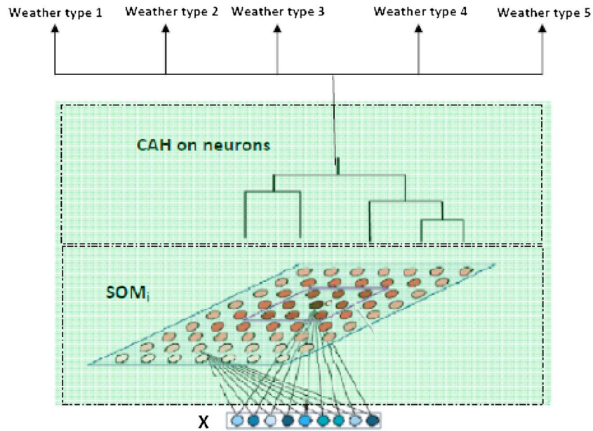
Figure 3. Schematic representation of the method and the structure of the SOM_i map ( i=1 for Banizoumbou, Niger, and i=2 for Cinzana, Cinzana). The network comprises two layers: an input layer used to present the observations and an adaptation layer for which a neighborhood constrains is defined (distance d between neurons and a neighborhood function). Each input vector ( X ) of SOM_i is thus constituted by 17 vertical profiles of atmospheric parameters (temperature, meridional, and zonal wind components at nine vertical levels) at each of the 17 grid meshes (Figure 2). The 459 ( 9 \times 3 \times 17 ) components of the input vector of SOM_i are output of the ECMWF forecast model analysis. Each neuron i of the map is fully connected to the input layer. It is associated with a group that is represented by a reference vector rv which is represented by the weights of the connection to the input layer. The neurons are clustered in classes by a hierarchical ascendant classification.
