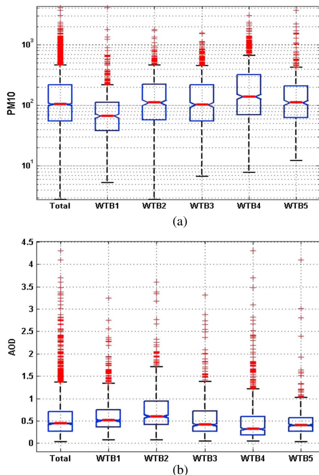
Figure 10. Statistical distribution of (a) PM 10 (μg/m 3 ) and (b) AOD for the complete data set and for the different weather types at Banizoumbou (Niger). The box represents the lower quartile (Q25—lower bar), the median value (middle bar), and the upper quartile (Q75—upper bar) of the studied variable. The T lines delineate the 9th percentile (lower T) and the 91th percentile (upper T) values, respectively.
