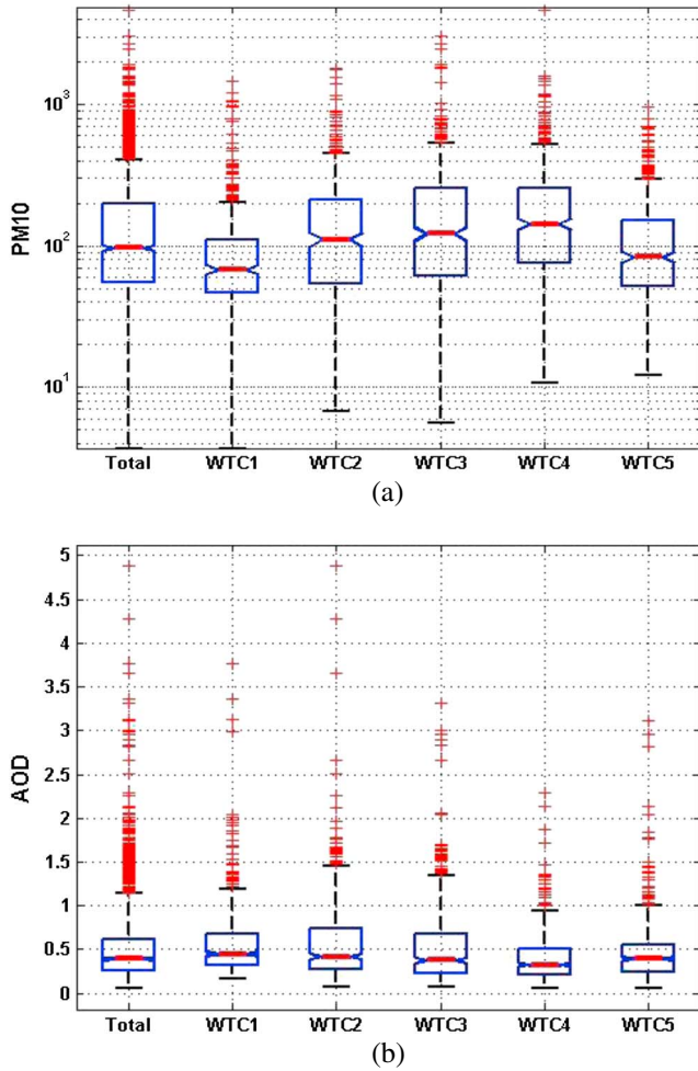
Figure 11. Statistical distribution of (a) PM 10 (µg/m 3 ) and (b) AOD for the complete data set and for the different weather types at Cinzana (Mali). The box represents the lower quartile (Q25—lower bar), the median value (middle bar), and the upper quartile (Q75—upper bar) of the studied variable. The T lines delineate the 9th percentile (lower T) and the 91th percentile (upper T) values, respectively.
