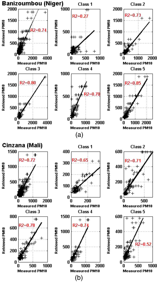
Figure 14. Scatterplot of the PM_{10} retrieval (measured PM_{10} versus retrieved PM_{10} from AOD) for the learning set and the test set for each weather types at the two stations ((a) Banizoumbou and (b) Cinzana) and for aggregating the results of the different classes for the whole studied period.
