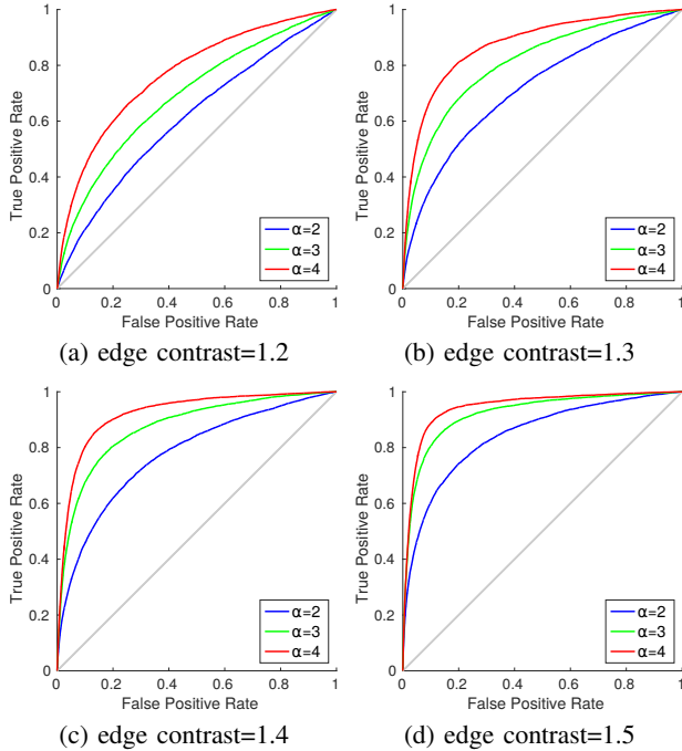
Fig. 2: ROC curves [28], [29] obtained using GR as an edge detector over several 1-look images with different edge contrasts values, and different values of \alpha .
