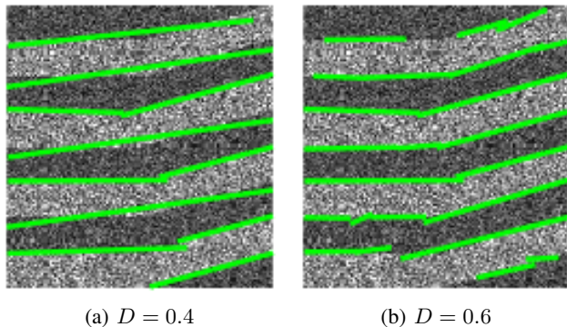
Fig. 6: Line segment detection results on 3-look synthetic edge images (contrast 1.6) for two different values of D . The angle difference of the problematic line segments is 16 degrees, while the angle tolerance is 22.5 degrees.
