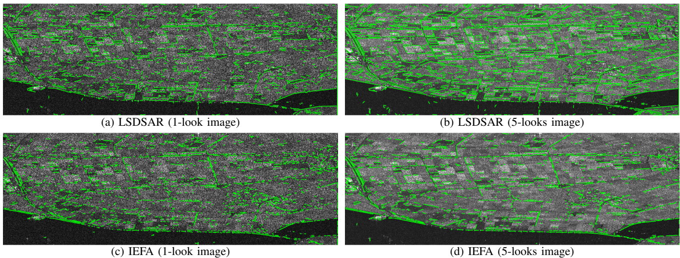
Fig. 11: Line segment detection using LSDSAR (first row) and IEFA (second row) over a 1-look (first column) and a 5-looks (second column) Sentinel 1 SAR images (Leystad).
