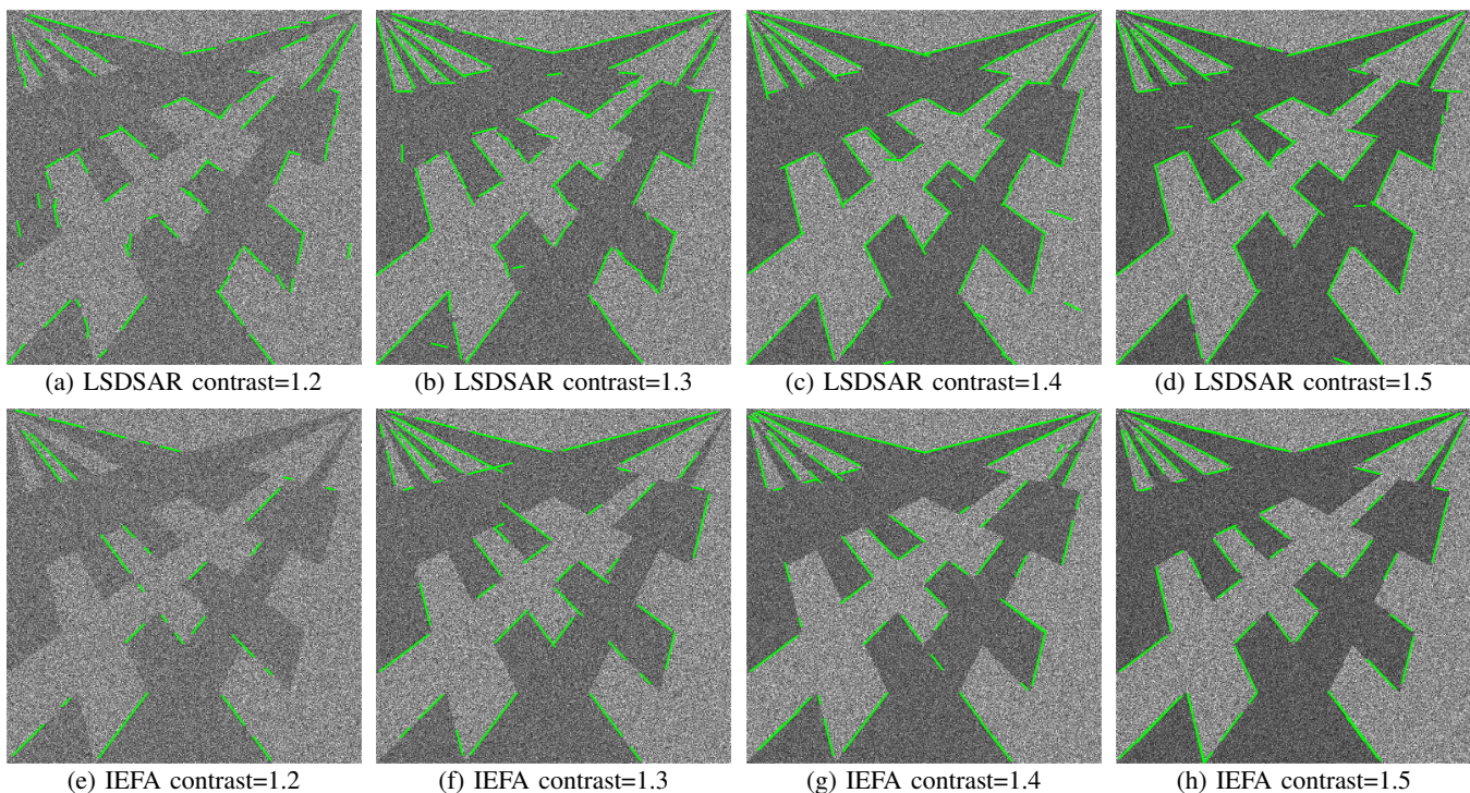
Fig. 8: Detection results obtained using LSDSAR (first row) and IEFA (second row) over a synthetic edge image with different contrast values (ranging between 1.2 and 1.5) corrupted with a speckle noise (3-look situation).
