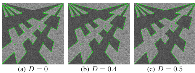
Fig. 5: Line segment detection on 3-look synthetic edge image (contrast 1.6) for different value of the density threshold.
