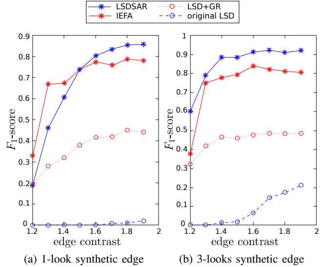
Fig. 7: Performances evaluations in terms of F_1 -score of the four algorithms, using a synthetic edge image with different contrast values (ranging between 1.2 and 1.9) and different levels of speckle noise (1-look in (a) and 3-look in (b)).
