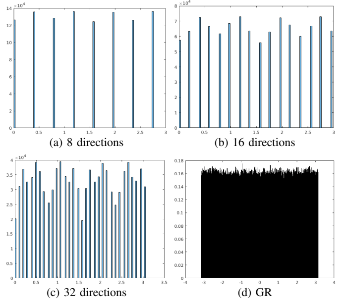
Fig. 1: Histograms of the local orientations computed over a 1-look pure speckle noise image of size 1024 \times 1024 pixels, using the multi-directional ratio based methods (a,b,c) or GR (d), with the same setting \alpha = 4 for all methods.
