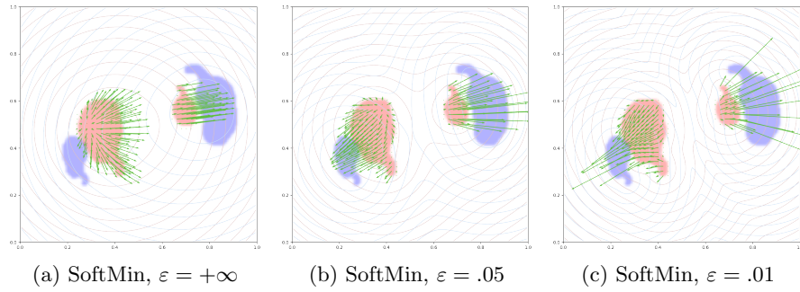
Fig. 6: The log-kernel fidelity interpolates between the Energy Distance and a weighted Hausdorff distance between the supports [1]. Here, we use the simple Euclidean cost C(x, y) = \|x - y\| .
