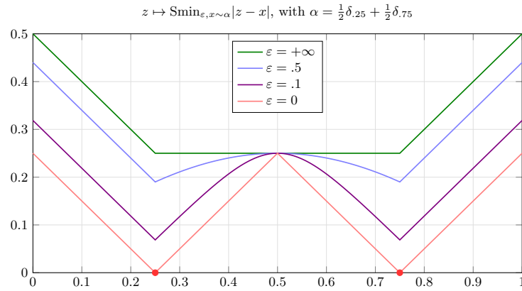
Fig. 5: The SoftMin operator. The log-sum-exp trick allows us to interpolate between the “Energy potential” |\cdot| \star \alpha – for \varepsilon = +\infty – and the distance field to the support \{.25, .75\} of \alpha – for \varepsilon = 0 .
