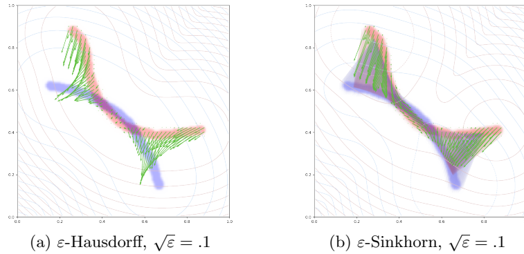
Fig. 10: Computing \varepsilon -Hausdorff and \varepsilon -Sinkhorn divergences. On this page, we use a quadratic cost C(x, y) = \|x - y\|^2 so that \varepsilon is homogeneous to a squared distance.
