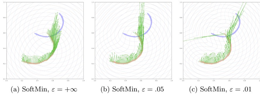
Fig. 7: Naive projection isn’t the panacea. Shape registration isn’t always about projecting source points onto their nearest target neighbors... Presented in section 3, the Sinkhorn loop will let us introduce a mass repartition constraint into our algorithms.
