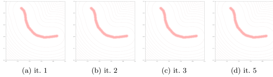
Fig. 8: The symmetric Sinkhorn algorithm converges fast. As we display the distance field a^{\alpha \leftrightarrow \alpha} – sampled on a uniform grid y_j – across the iterations of the symmetric Sinkhorn algorithm, we see that running it with n_{\text{its}} = 3 is enough for practical purposes.
