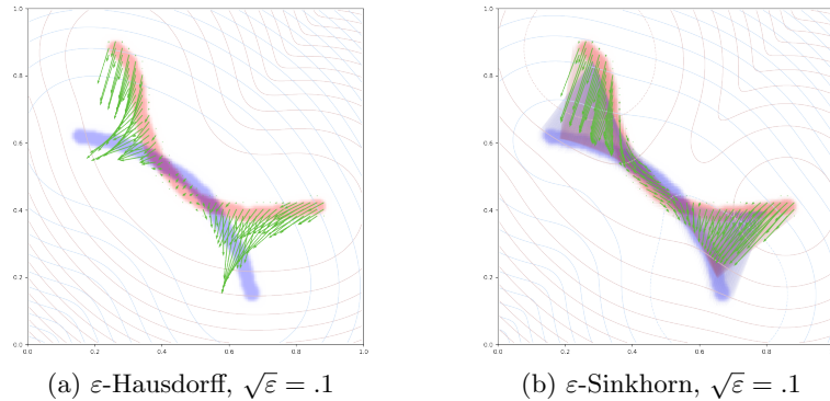
Fig. 10: Computing \varepsilon -Hausdorff and \varepsilon -Sinkhorn divergences. On this page, we use a quadratic cost C(x, y) = \|x - y\|^2 so that \varepsilon is homogeneous to a squared distance.
