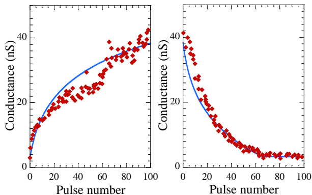
Figure 5. Evolution of the conductance for the devices from Michigan, fitted with the model D. Left: device conductance (measured at 1 V) after each pulse in a serie of potentiating ( V=-3.2 V) pulses. Right: same with depressing ( V=2.8 V) pulses. Diamond: experimental data, reproduced from [11]. Full line: Model D (parameters listed in Table I).
